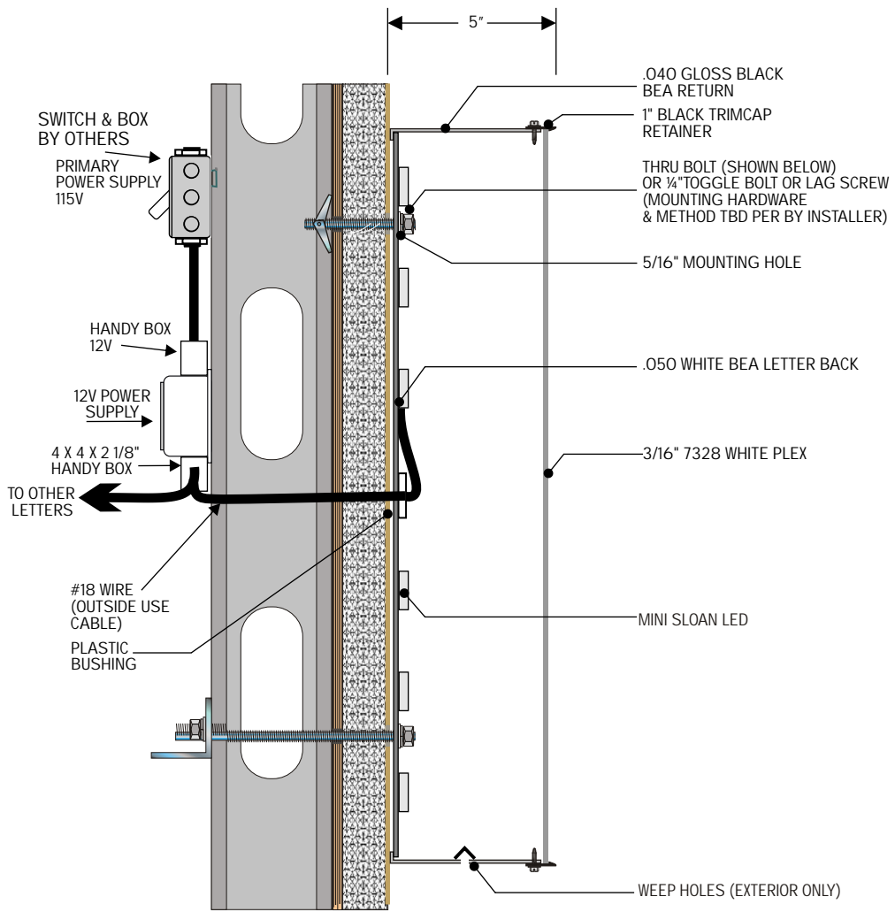
SECTION DETAIL FACE-LIT LED
