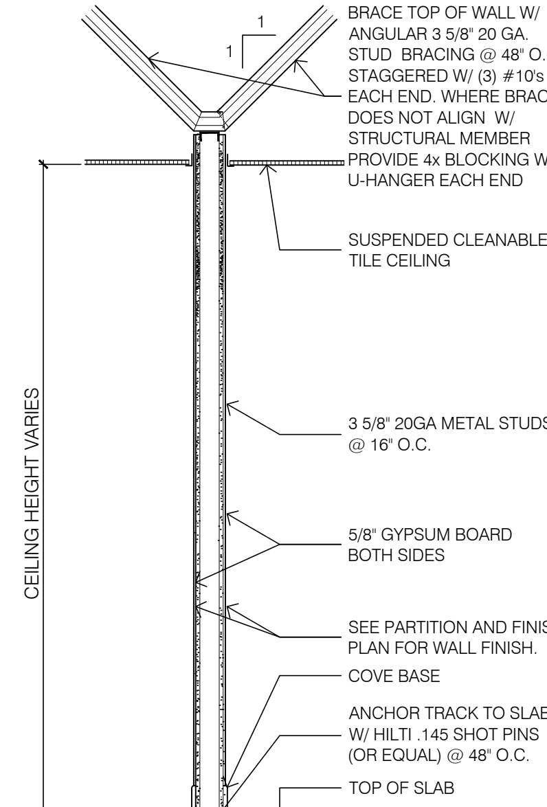
3 TYPICAL INTERIOR PARTITION SCALE: 1/2" = 1'-0"
