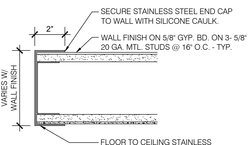
4 STAINLESS STEEL END CAP DETAIL SCALE: 3" = 1'-0"
