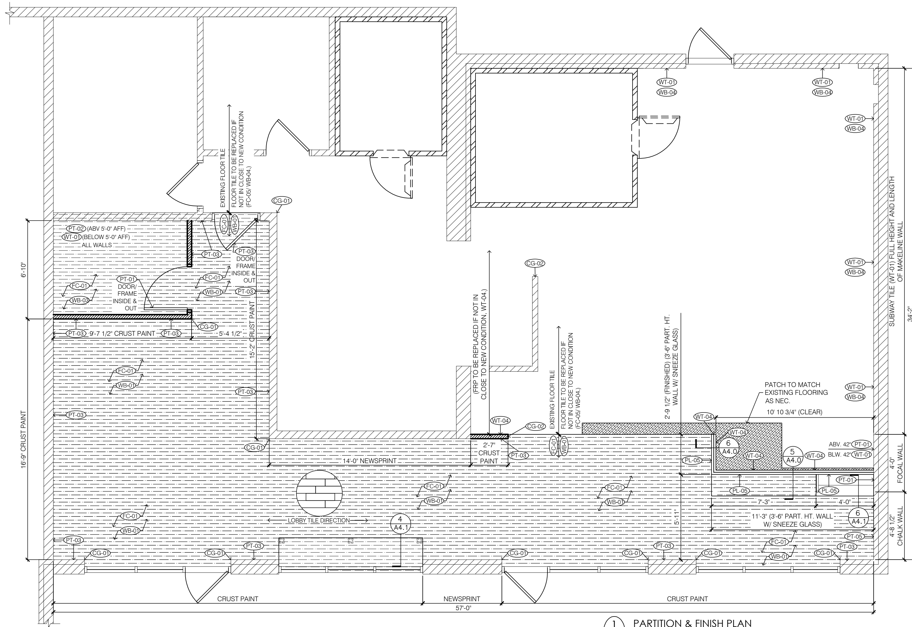
1 PARTITION & FINISH PLAN ALL DIMENSIONS TO FACE OF STUD UNLESS OTHERWISE NOTED SCALE: 1/4" = 1'-0"
