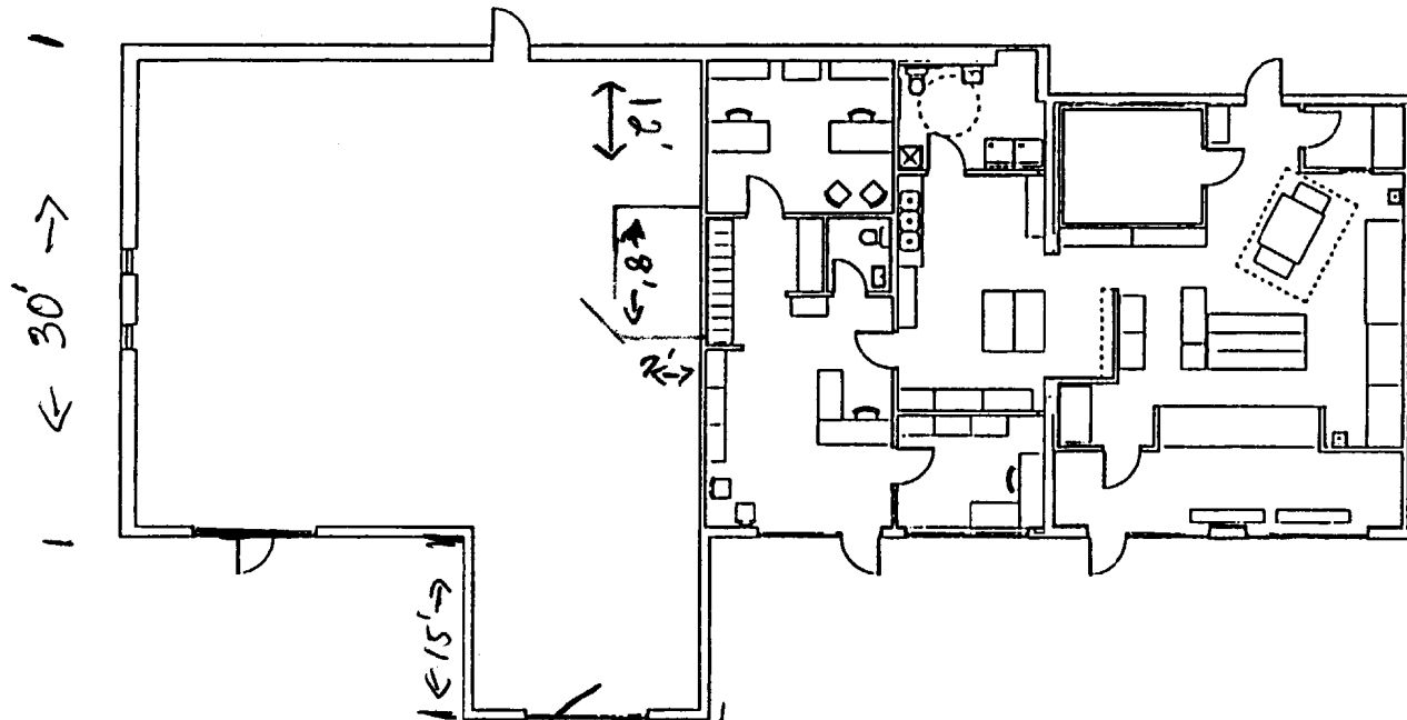
① FLOOR PLAN SCALE: 1/8" = 1'-0" 47'6" front door
