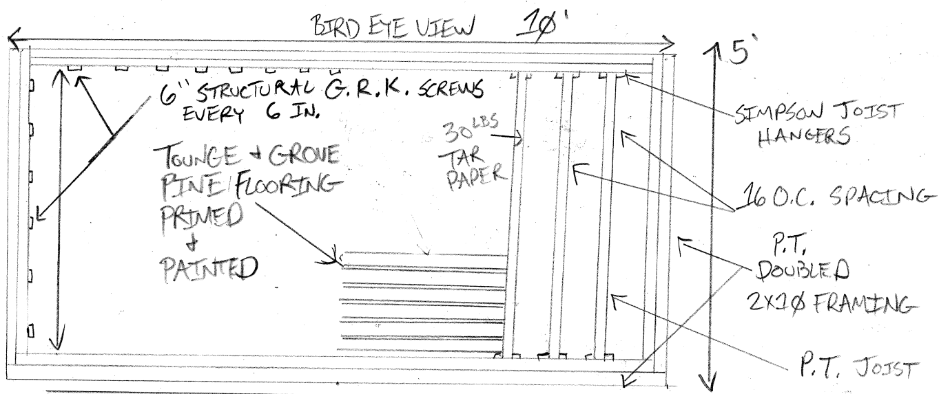
1/2 SCALE FRONT PORCH FRAMING WITH PRESSURE TREATED LUMBER
