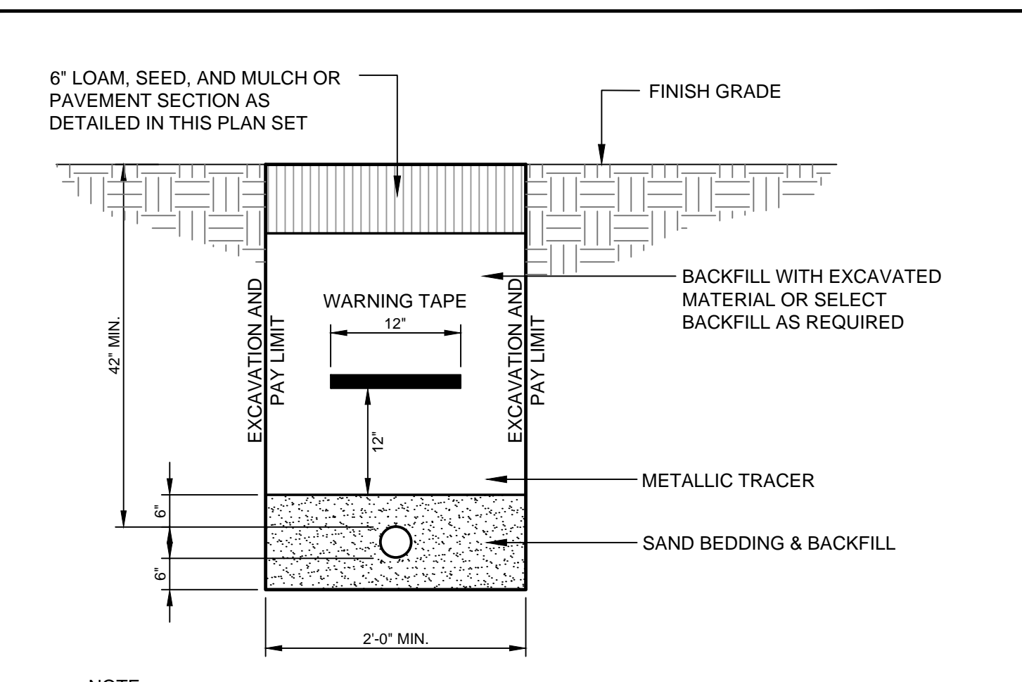
(E) GAS SERVICE TRENCH SECTION N.T.S.
