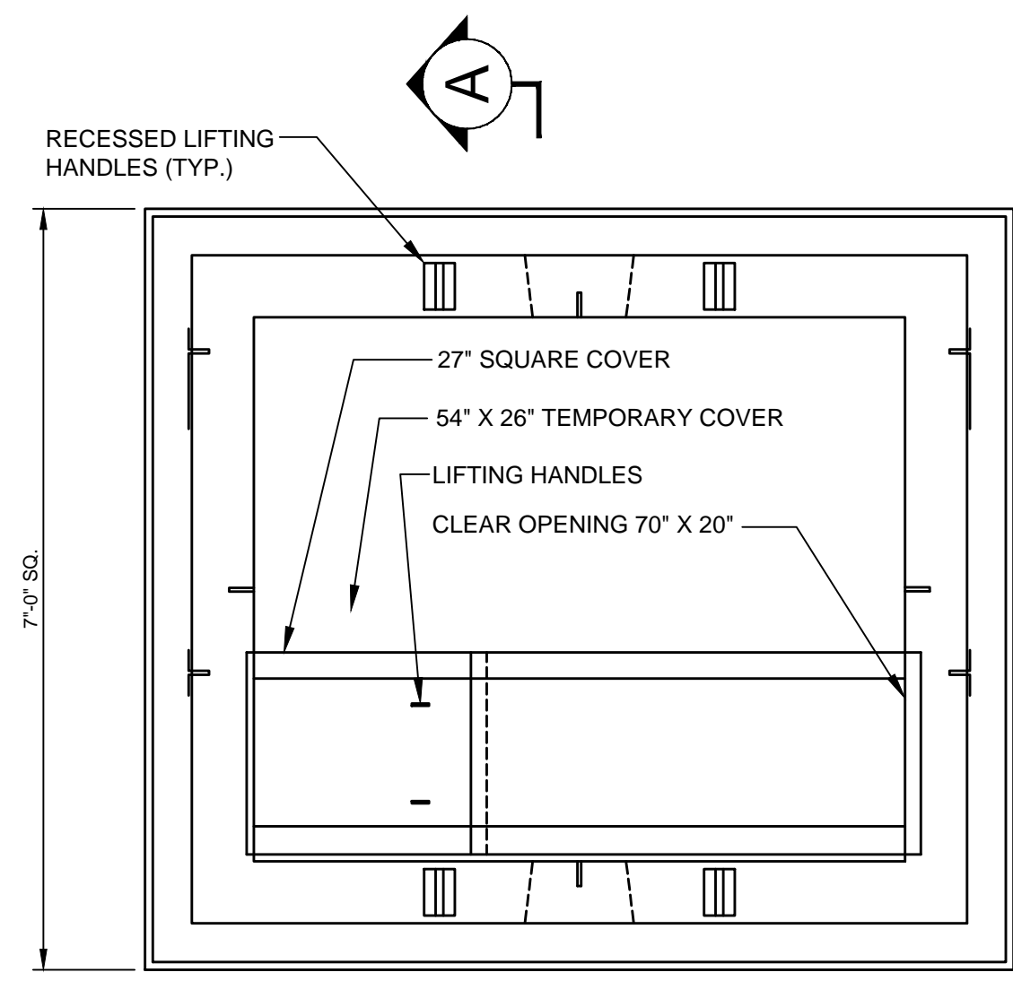
TOP VIEW
