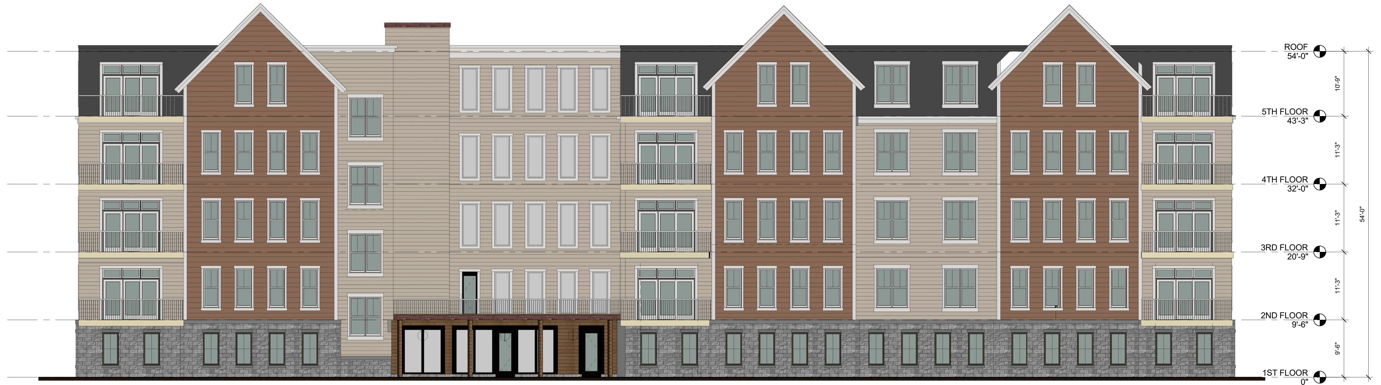
1 | SOUTH ELEVATION 1/8" = 1'-0" 0 2'-0" 4'-0" 8'-0" 16'-0"
