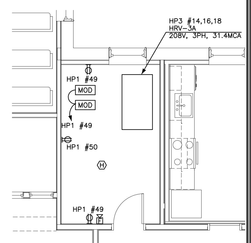
3 | ERV 3011 1/4" = 1'-0"
