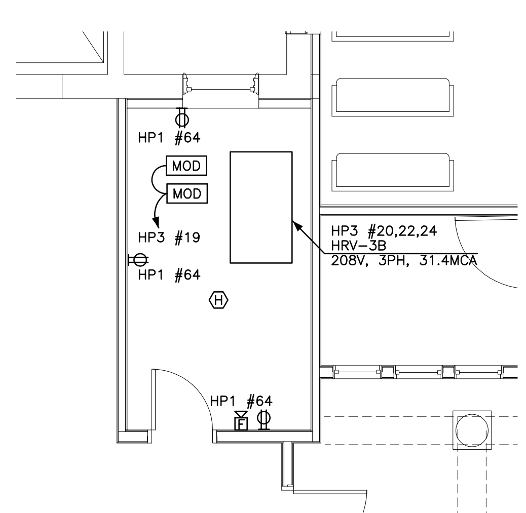
2 | ERV 3010 1/4" = 1'-0"
