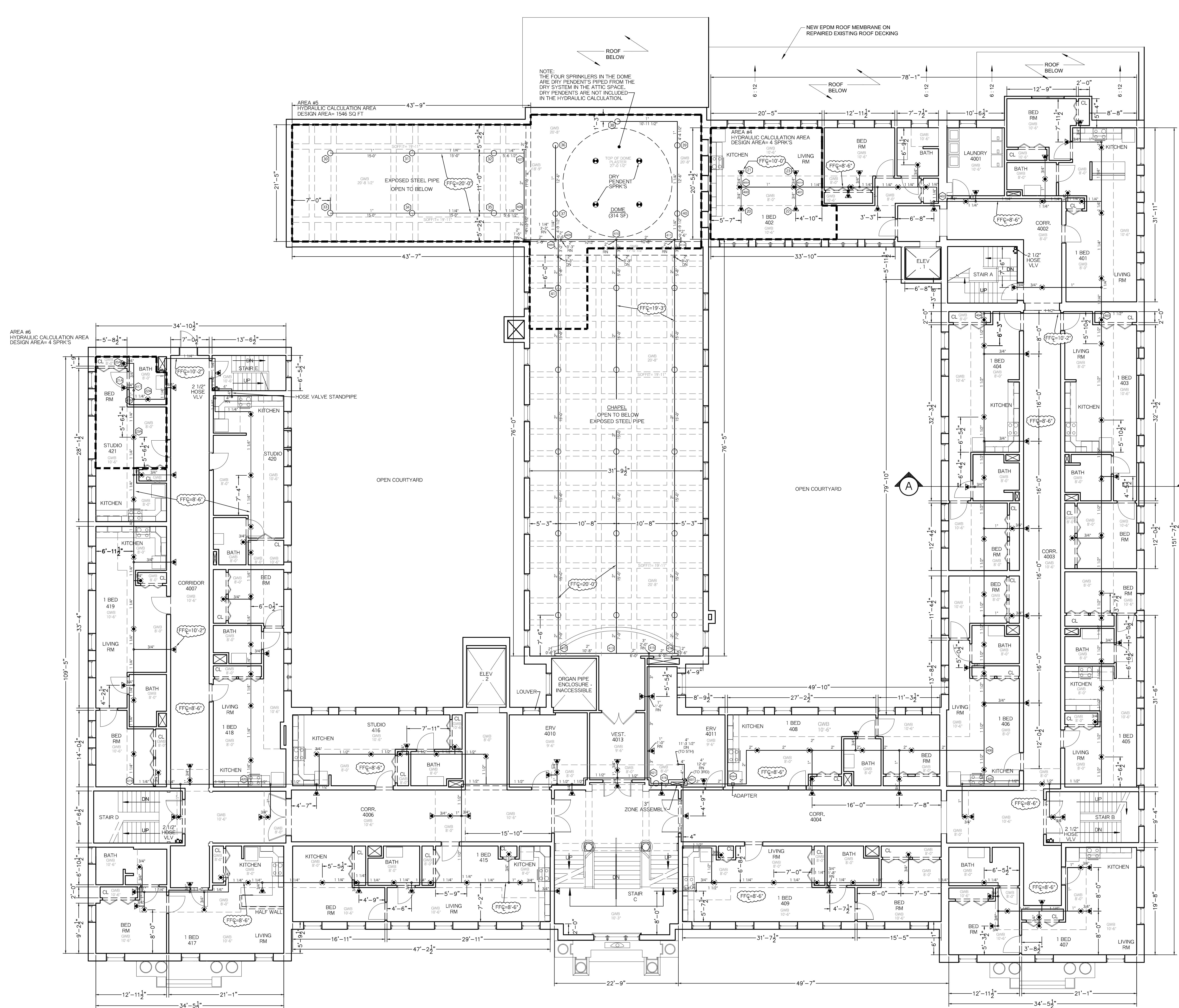
FOURTH FLOOR PLAN SCALE: 1/8" = 1'-0" FLR ELEV: 153'-5" TOTAL FLR AREA= 19,033 SF
