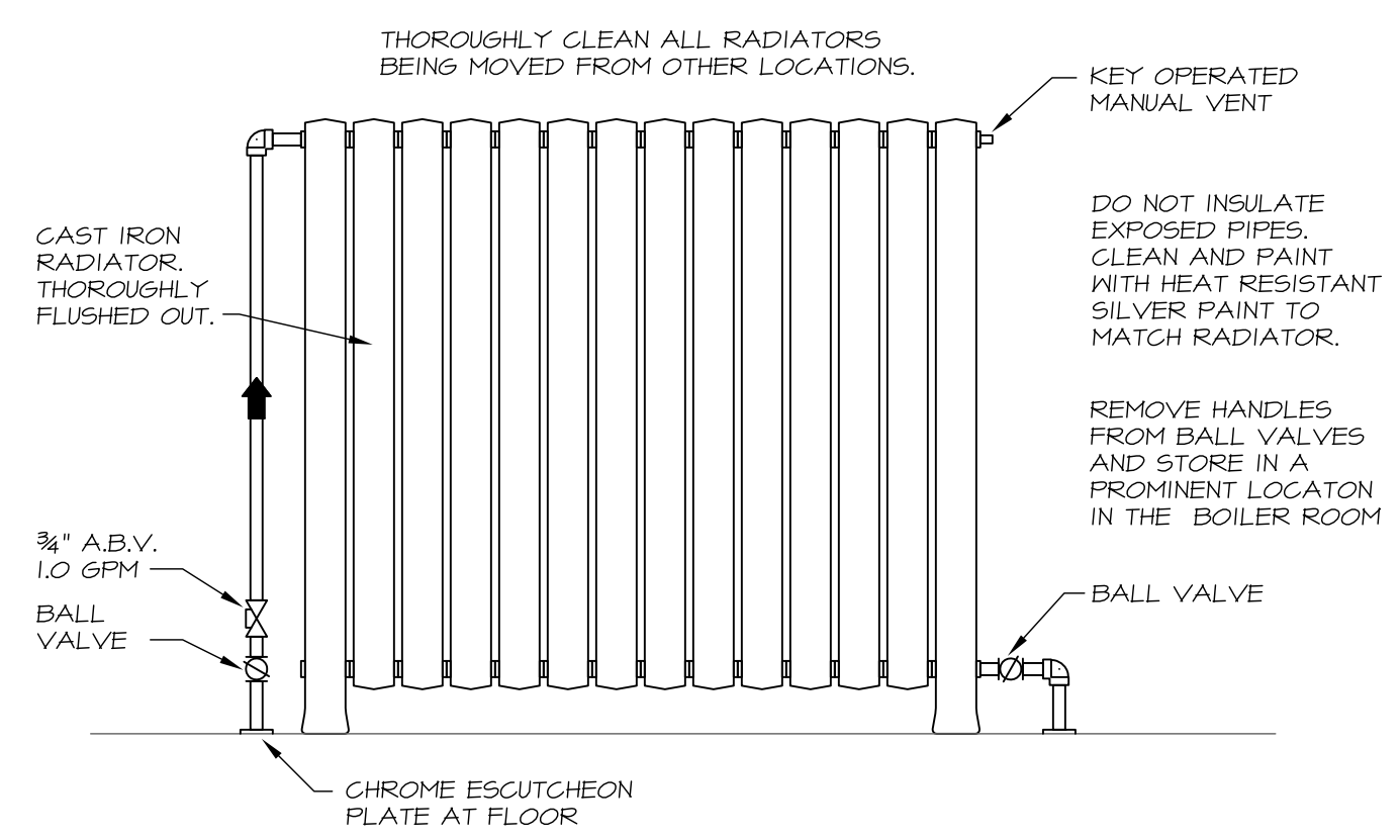
1 CAST IRON RADIATOR HOT WATER PIPING DETAIL NO SCALE
