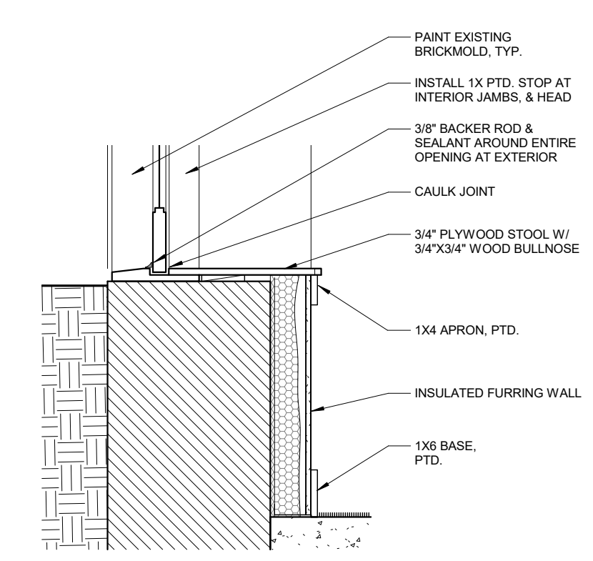
2 COURTYARD WINDOW SECTION 3/4" = 1'-0"
