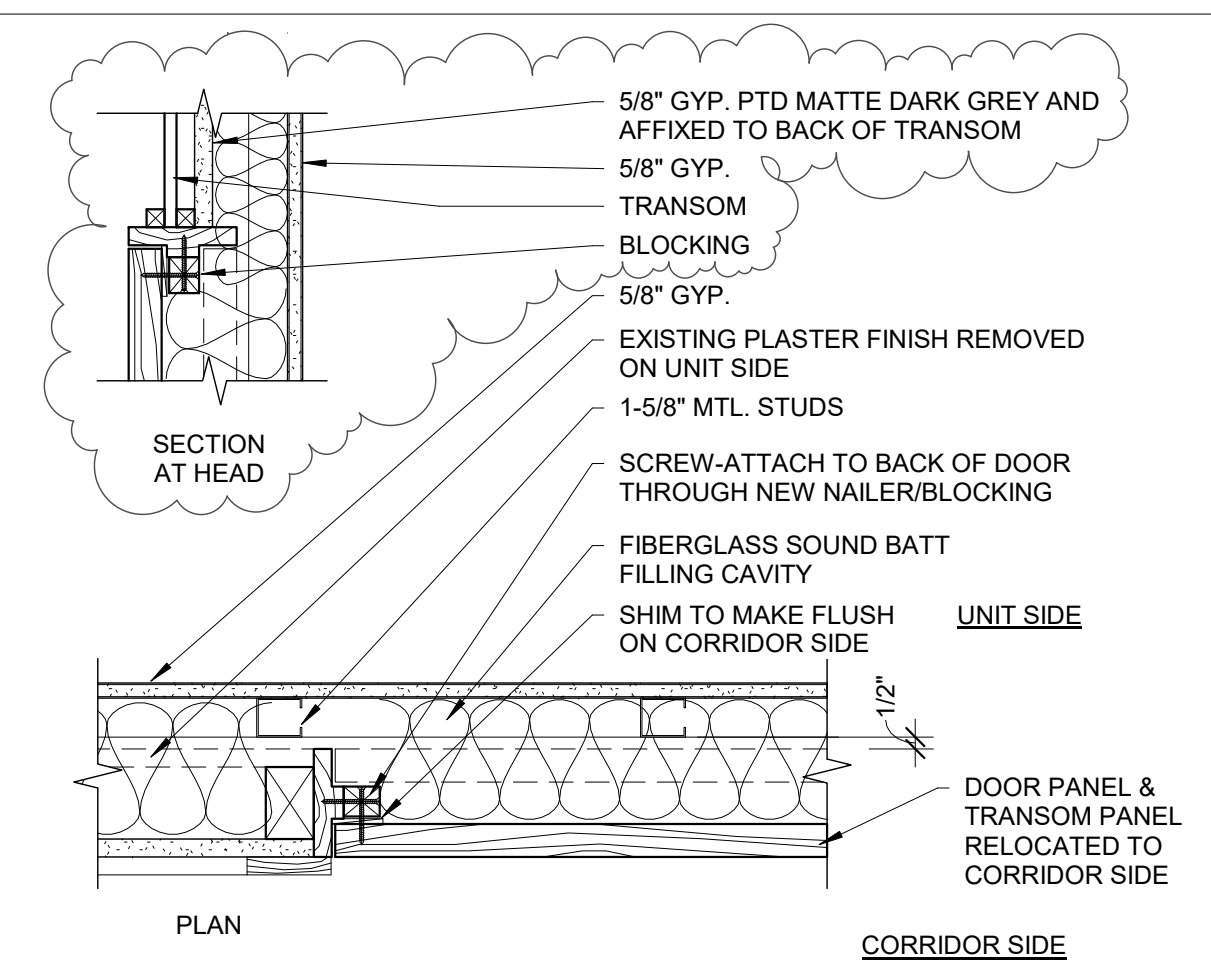
1 HISTORIC FIXED DOOR DETAIL 1 1/2" = 1'-0"
