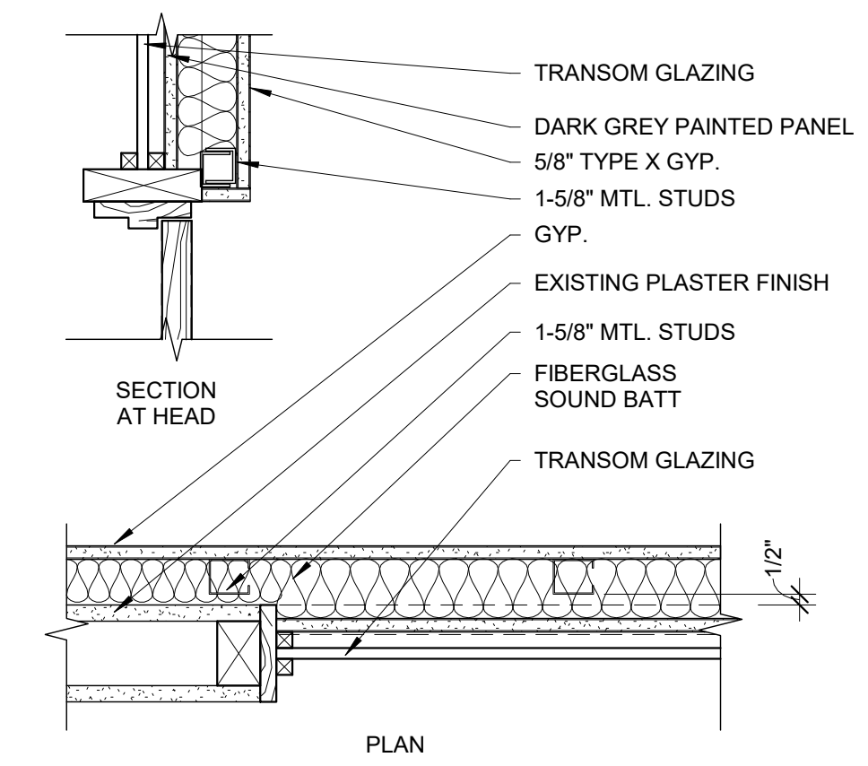
3 EXISTING TRANSOM RATING DETAIL 1 1/2" = 1'-0"
