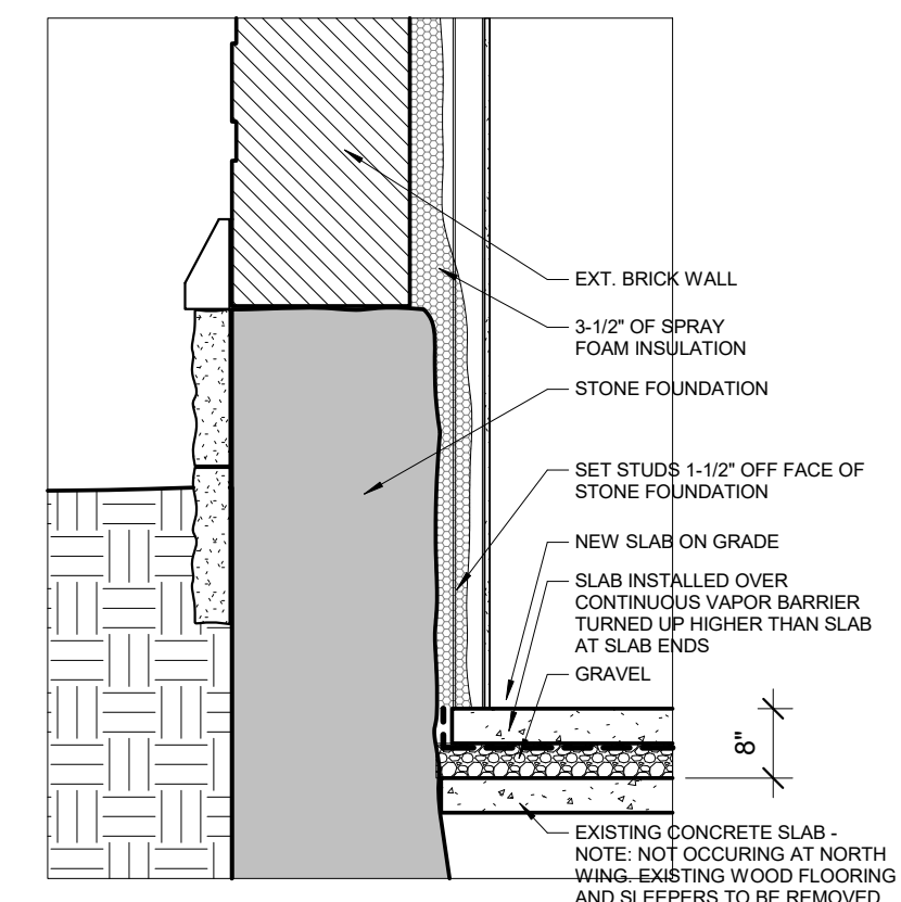
2 NEW FURRING WALL AT EXIST. MASONRY 1/2" = 1'-0"
