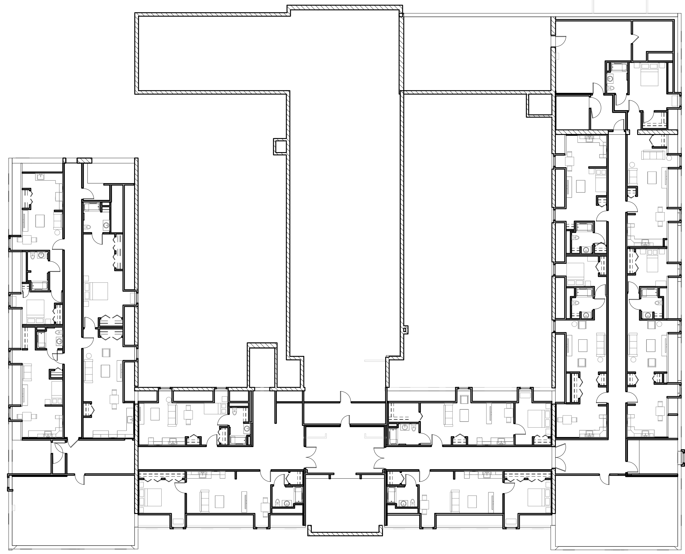
1 | FIFTH FLOOR LIFE SAFETY 1/16" = 1'-0"
