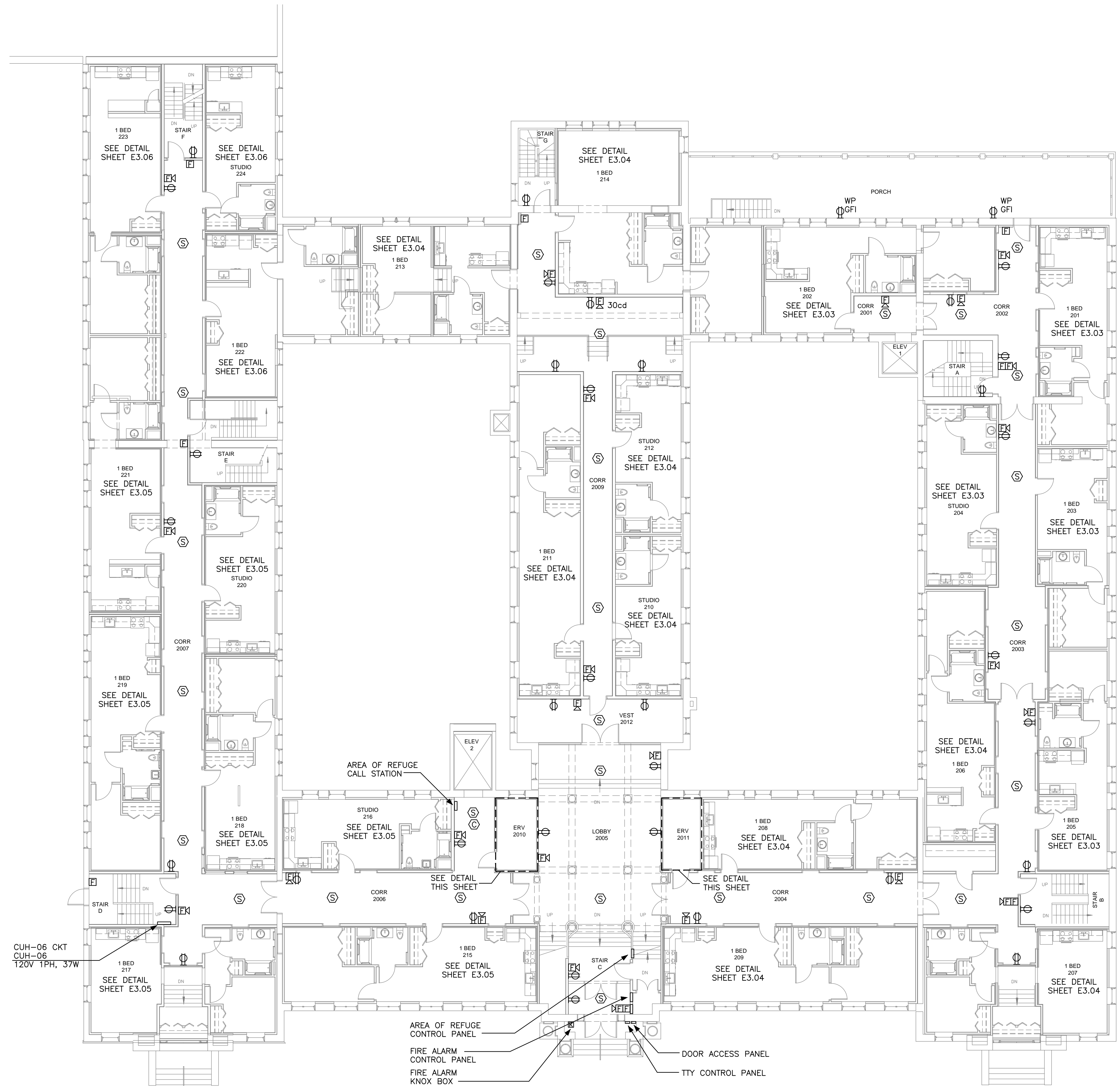
1 | SECOND FLOOR - POWER 1/4" = 1'-0"
