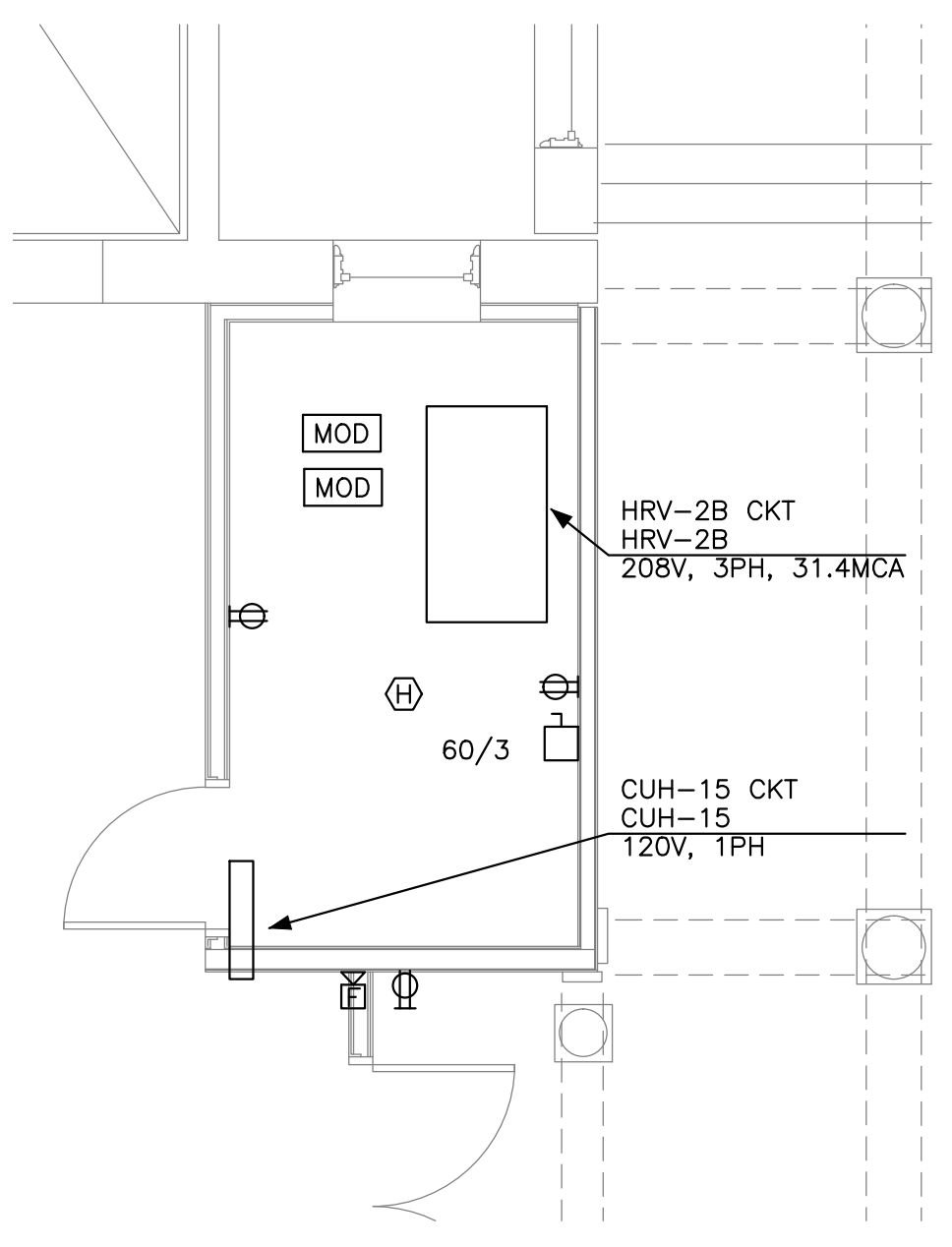
2 | ERV 2010 1/4" = 1'-0"
