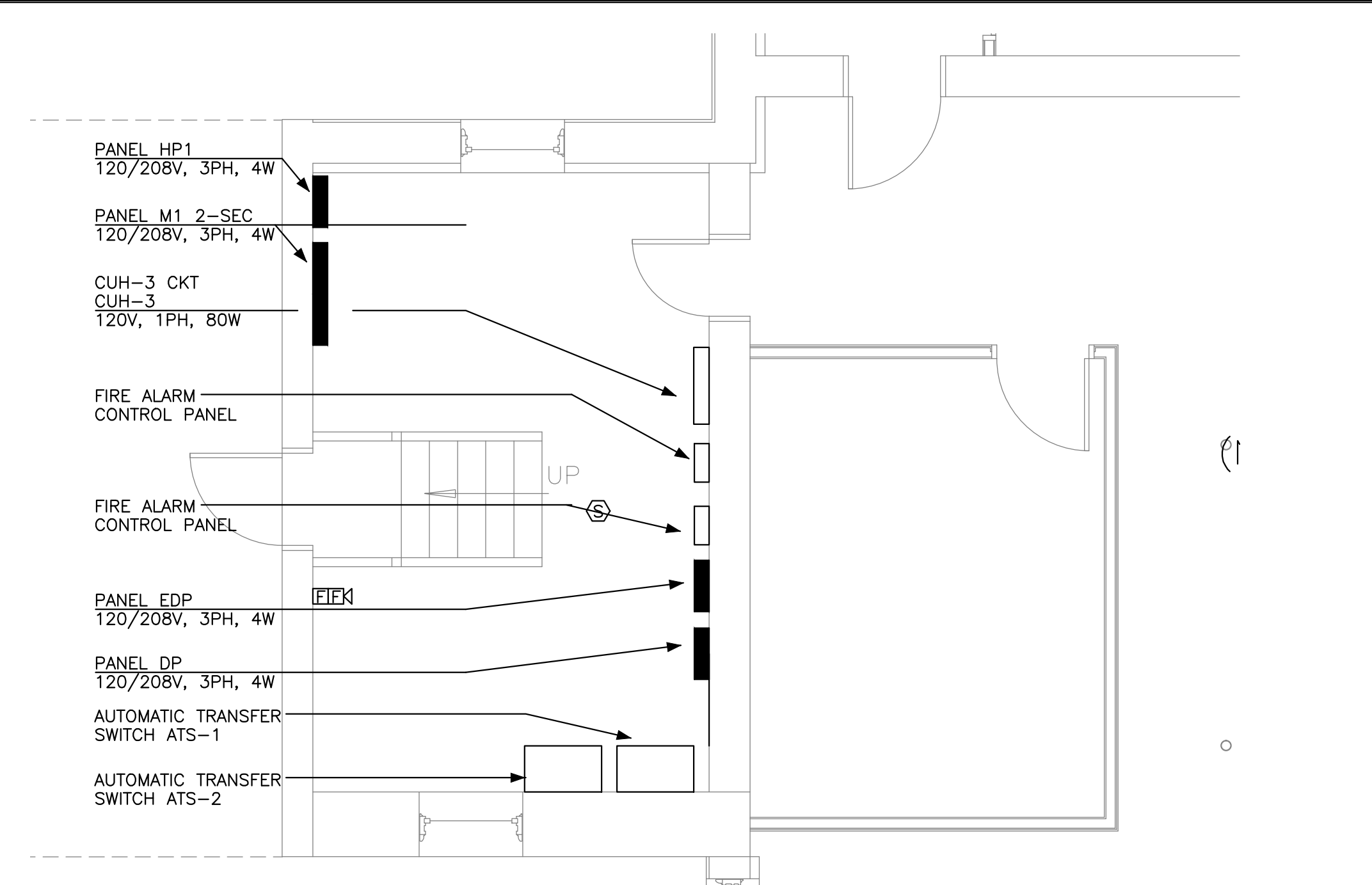
3 | ELEC 1021 & ELEC METERS 1018 1/4" = 1'-0"
