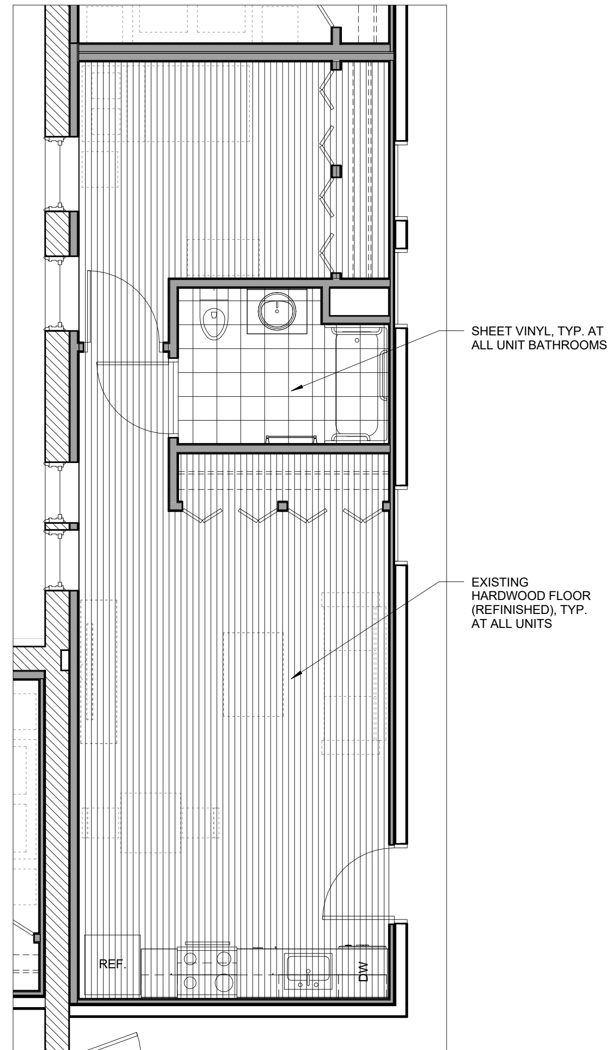
1 | TYP. UNIT FINISH PLAN 1/4" = 1'-0"
