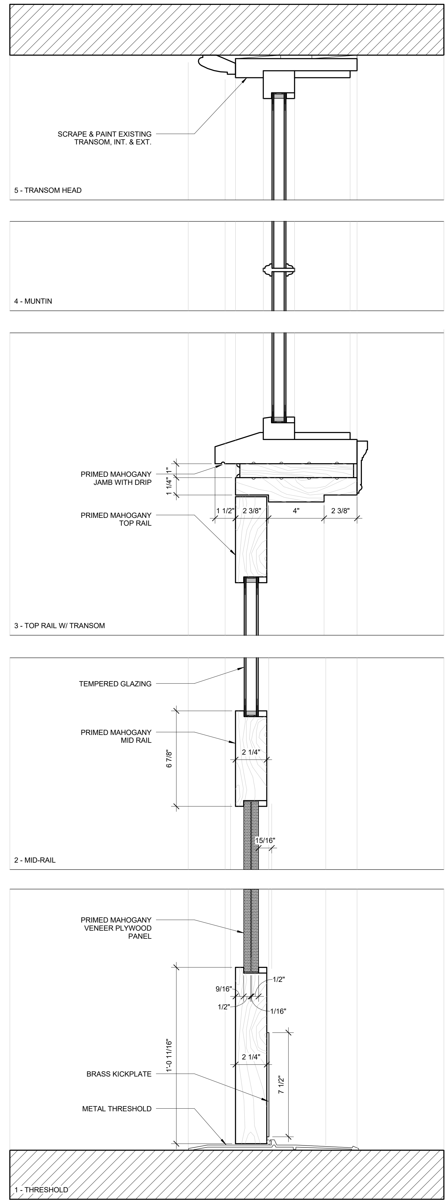
1 | WOOD STOREFRONT SECTION 3" = 1'-0"
