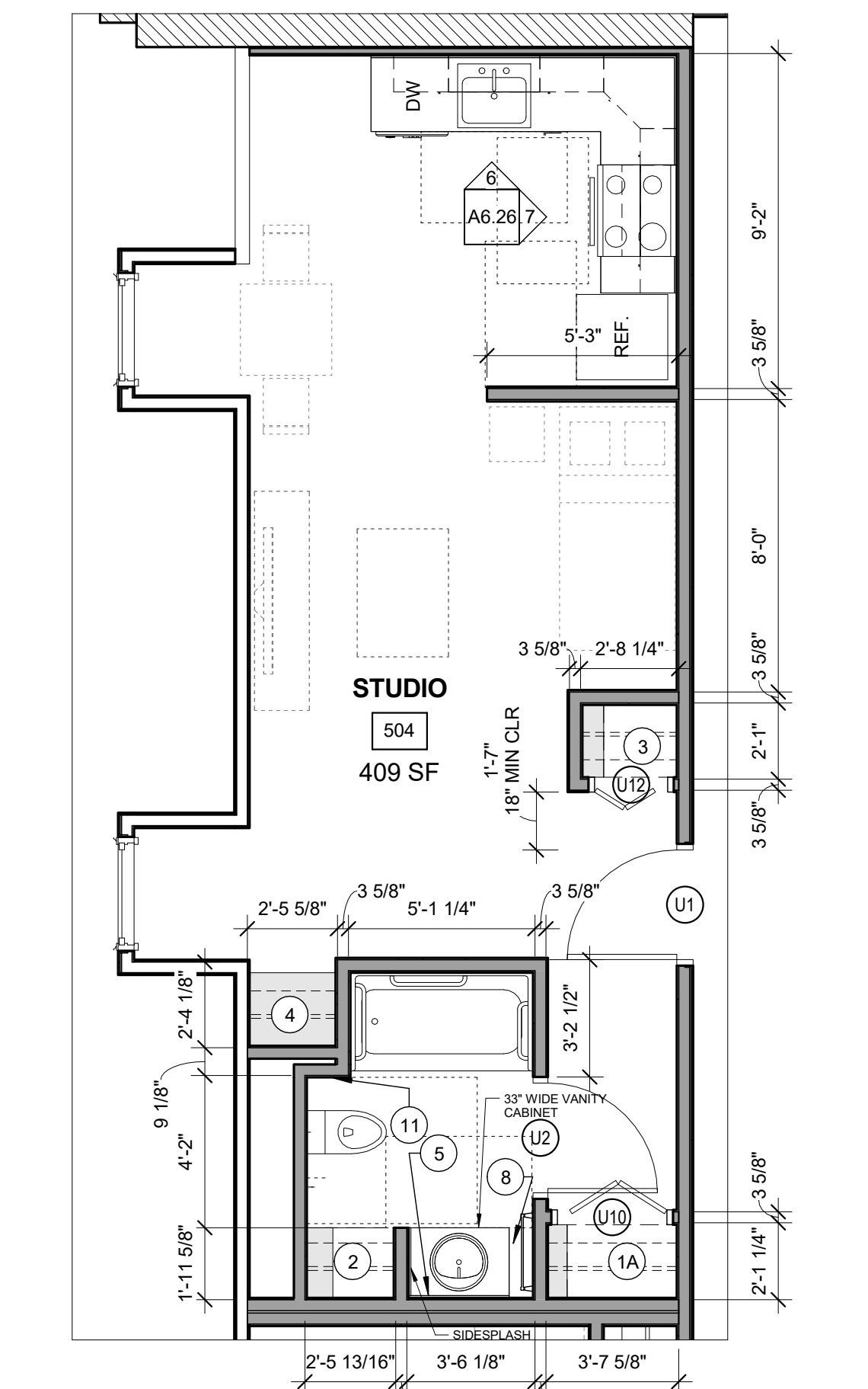
2 | UNIT 504 1/4" = 1'-0"
