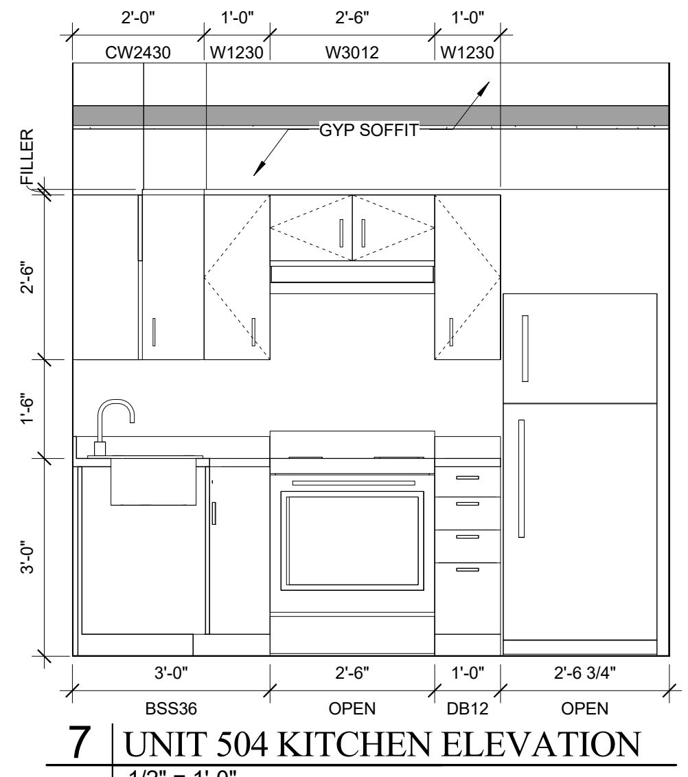
7 | UNIT 504 KITCHEN ELEVATION 1/2" = 1'-0"
