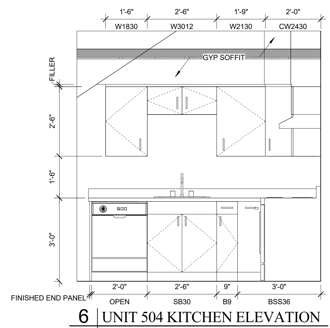
6 | UNIT 504 KITCHEN ELEVATION 1/2" = 1'-0"
