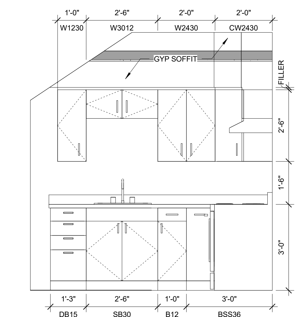
8 | UNIT 505 KITCHEN ELEVATION 1/2" = 1'-0"
