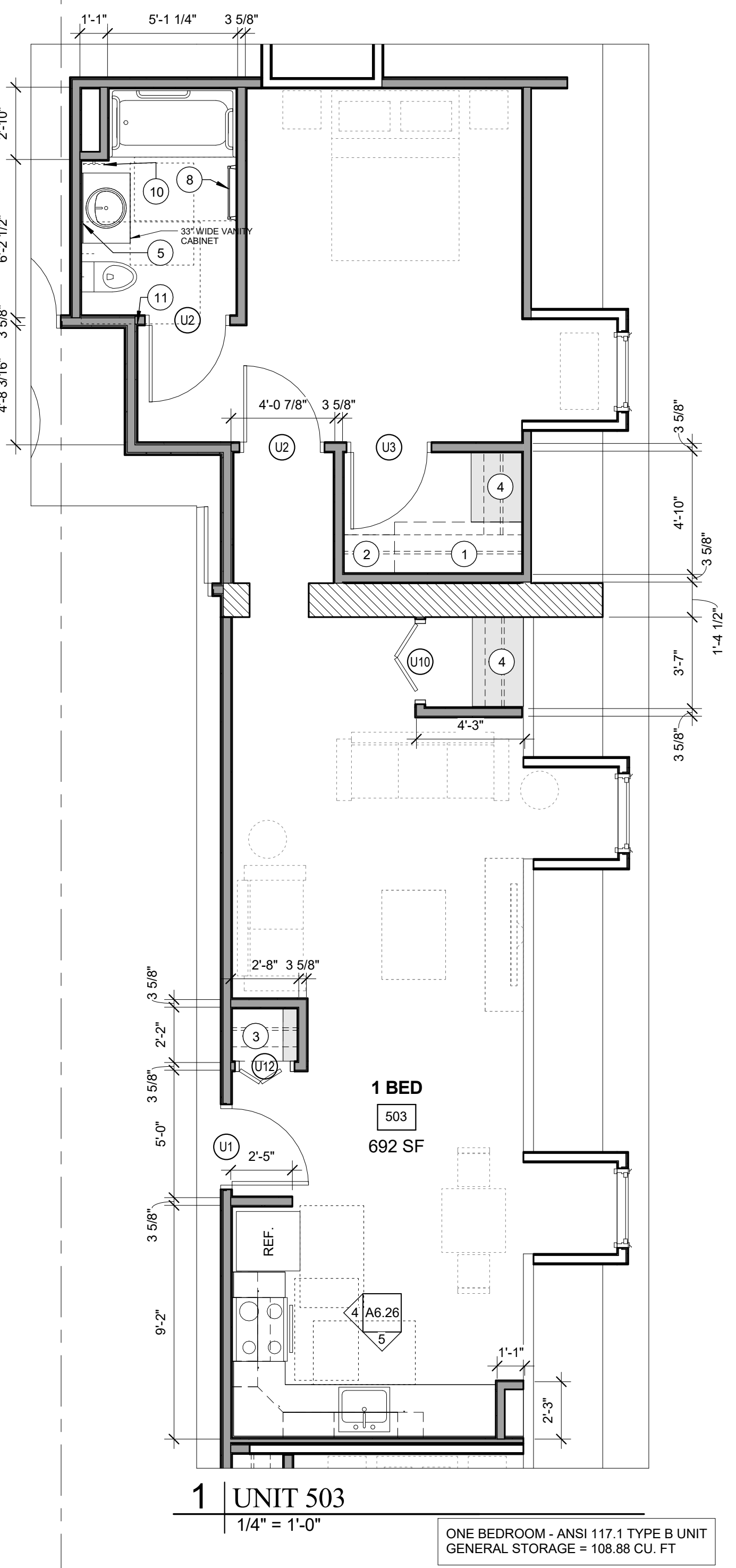
1 | UNIT 503 1/4" = 1'-0"
