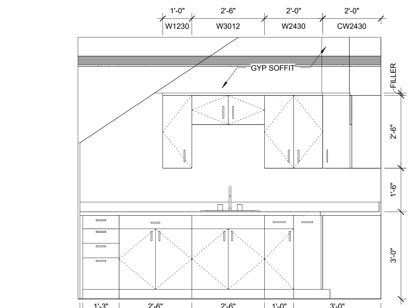
5 | UNIT 503 KITCHEN ELEVATION 1/2" = 1'-0"
