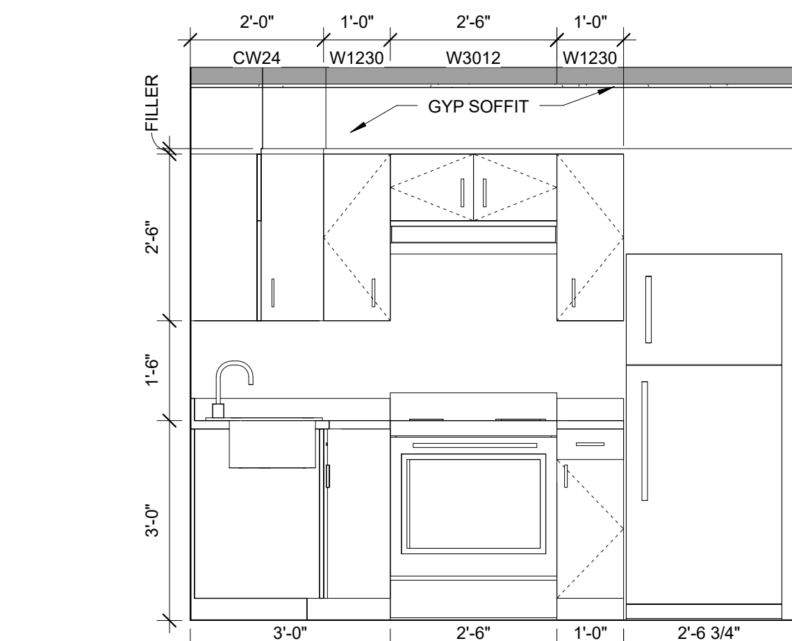
4 | UNIT 503 KITCHEN ELEVATION 1/2" = 1'-0"
