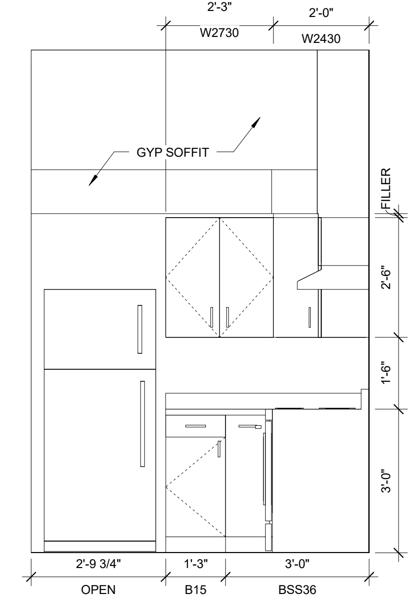
9 UNIT 421 KITCHEN ELEVATION 1/2" = 1'-0"
