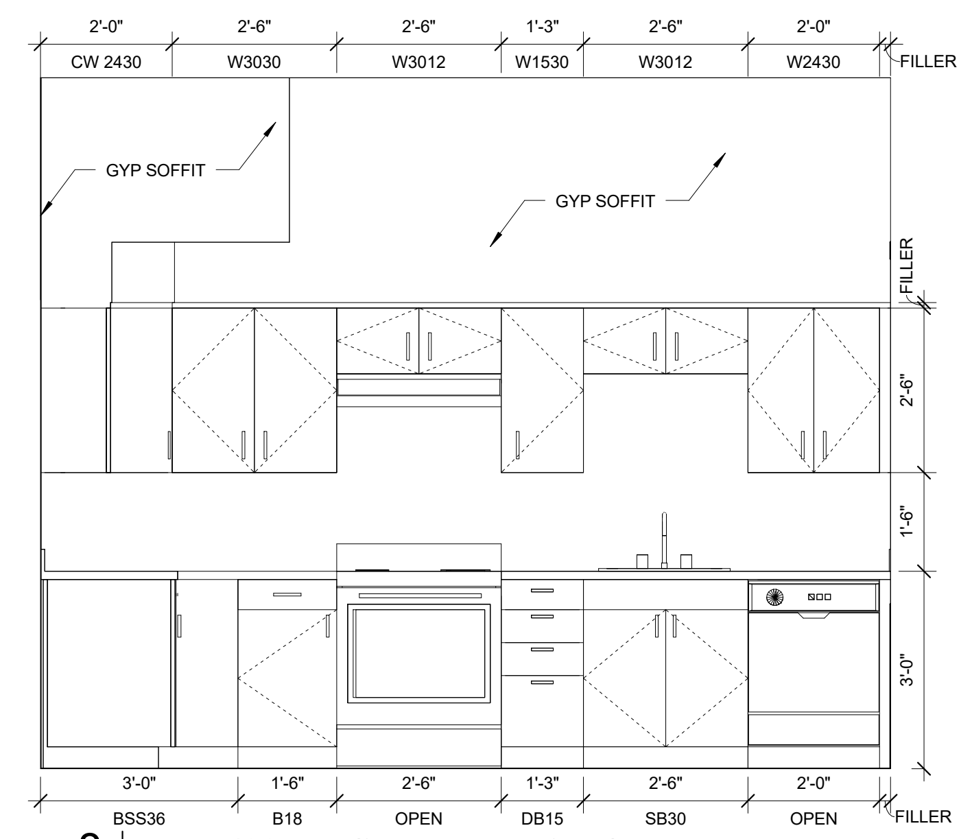
9 UNIT 421 KITCHEN ELEVATION 1/2" = 1'-0"
