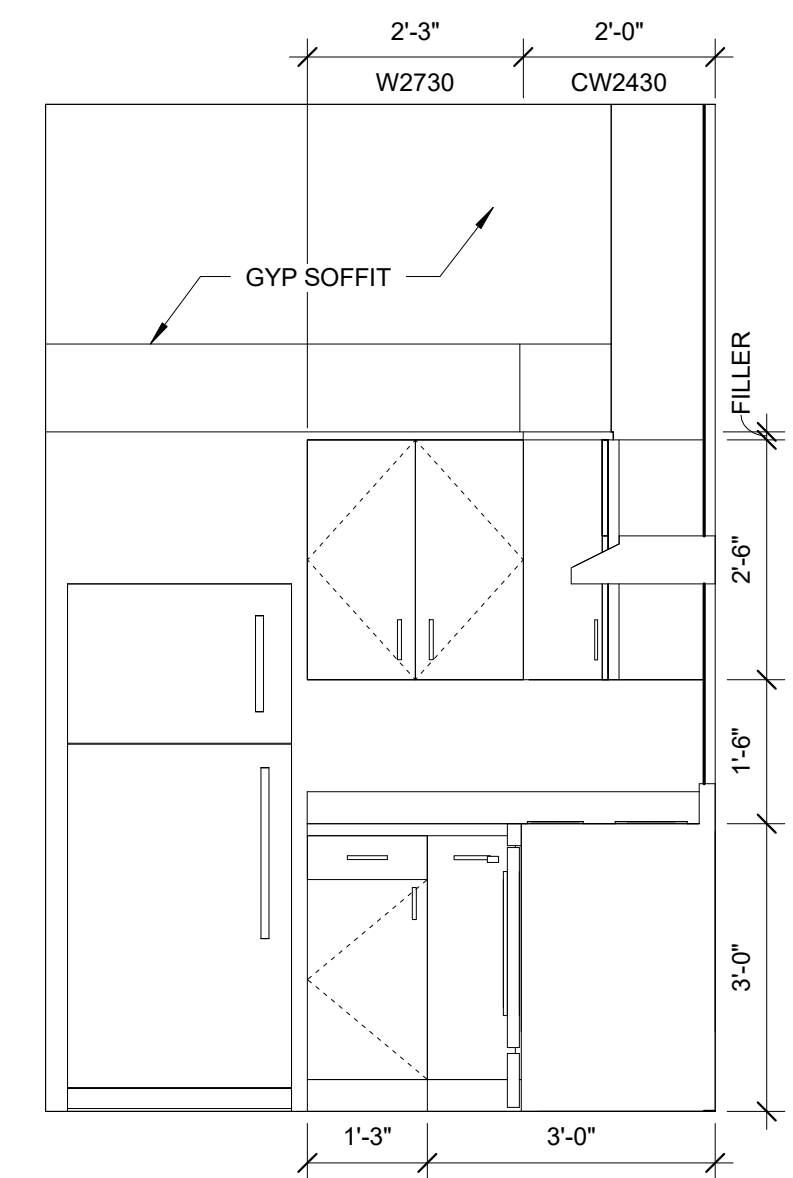
7 UNIT 420 KITCHEN ELEVATION 1/2" = 1'-0"
