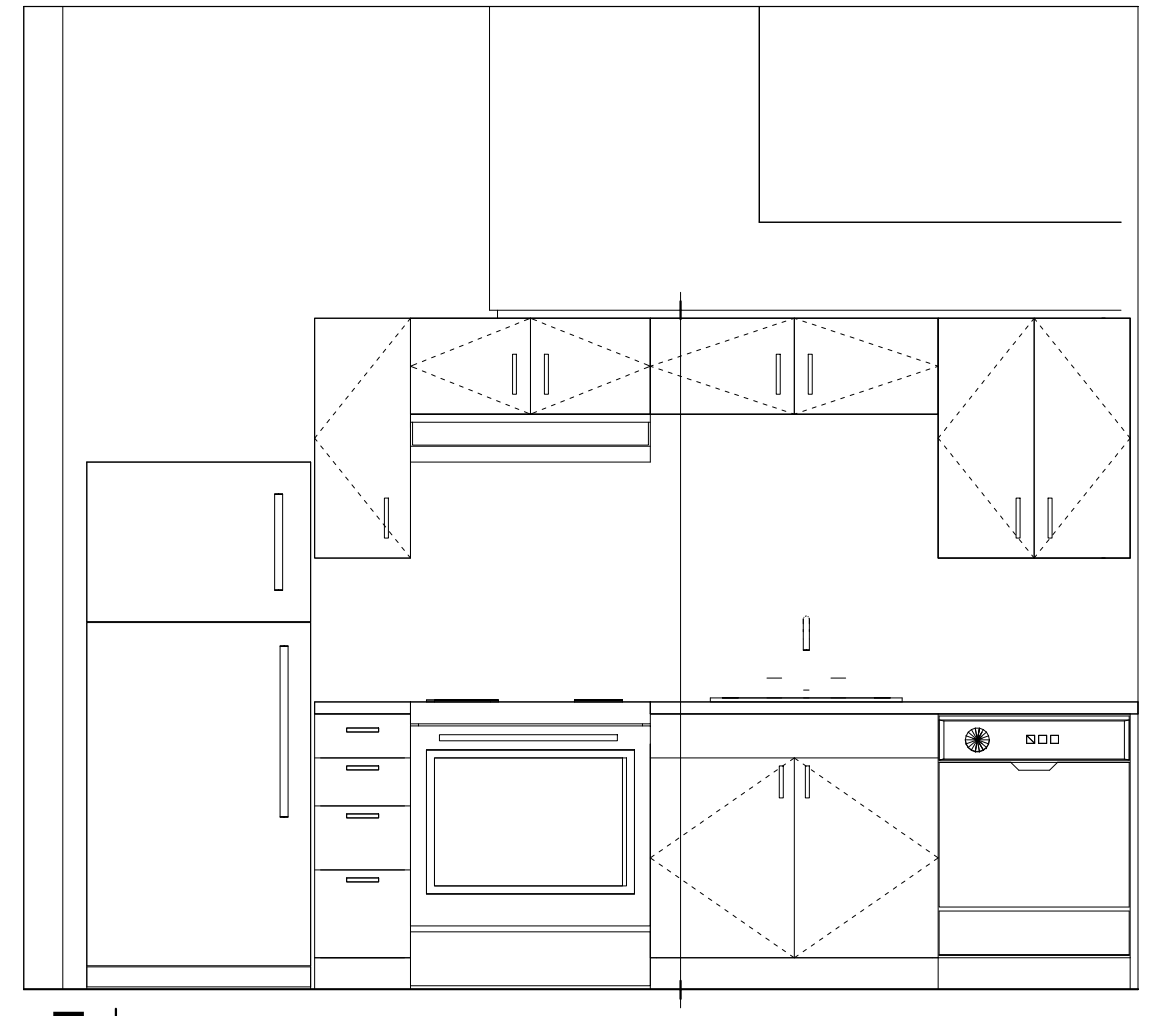
7 | UNIT 324 KITCHEN ELEVATION 1/2" = 1'-0"
