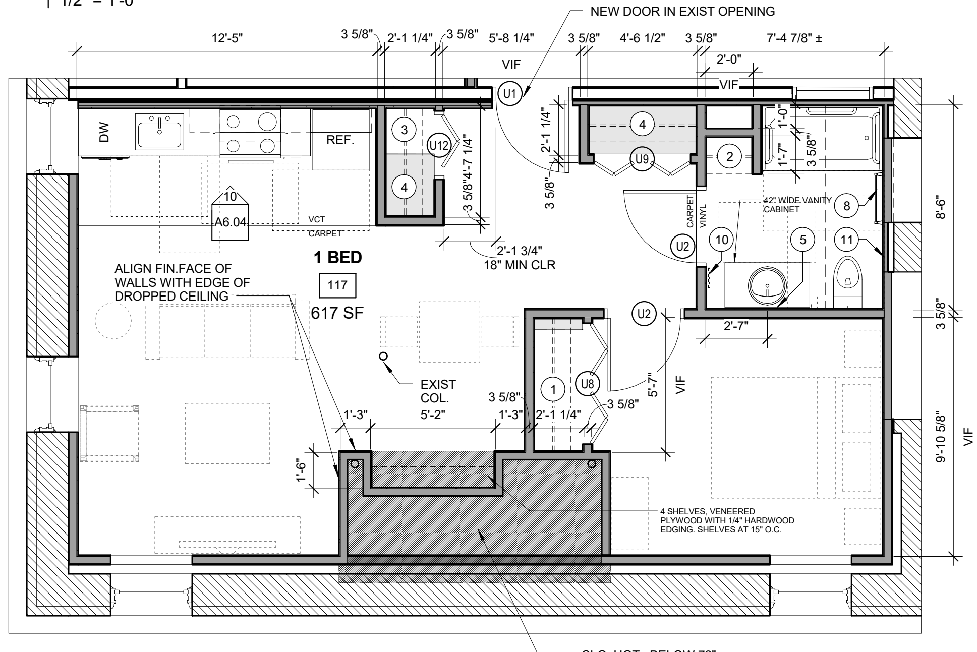
12 | UNIT 117 1/4" = 1'-0" ONE BEDROOM - ANSI 117.1 TYPE B GENERAL STORAGE = 119.3 CU.FT
