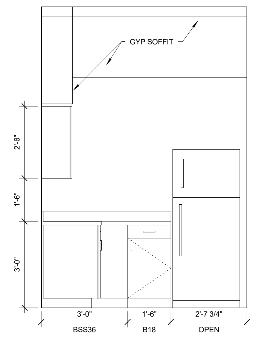
3 | UNIT 119 KITCHEN ELEVATION 1/2" = 1'-0"
