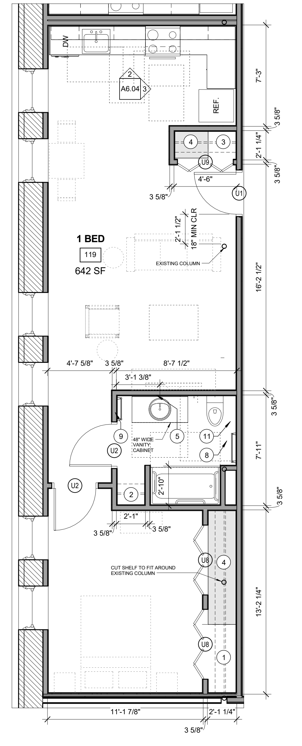
1 | UNIT 119 1/4" = 1'-0" ONE BEDROOM - ANSI 117.1 TYPE B GENERAL STORAGE = 168.5 CU.FT
