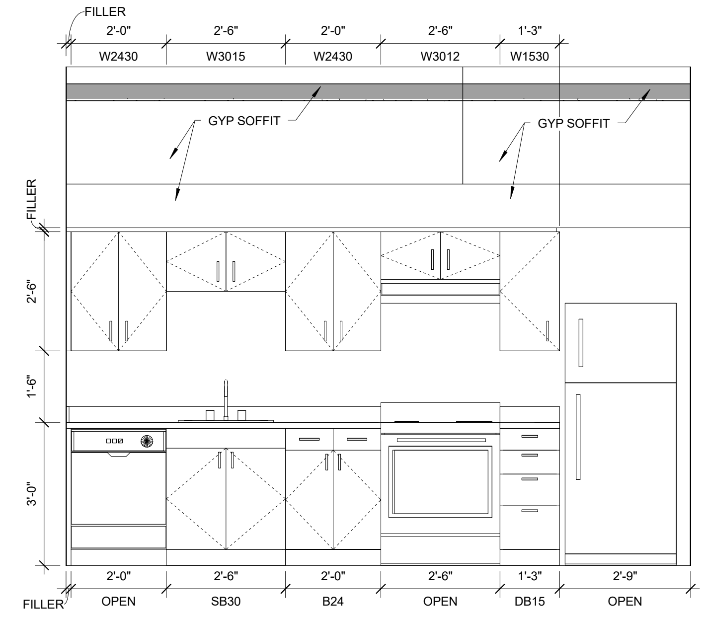
11 | UNIT 118 KITCHEN ELEVATION 1/2" = 1'-0"
