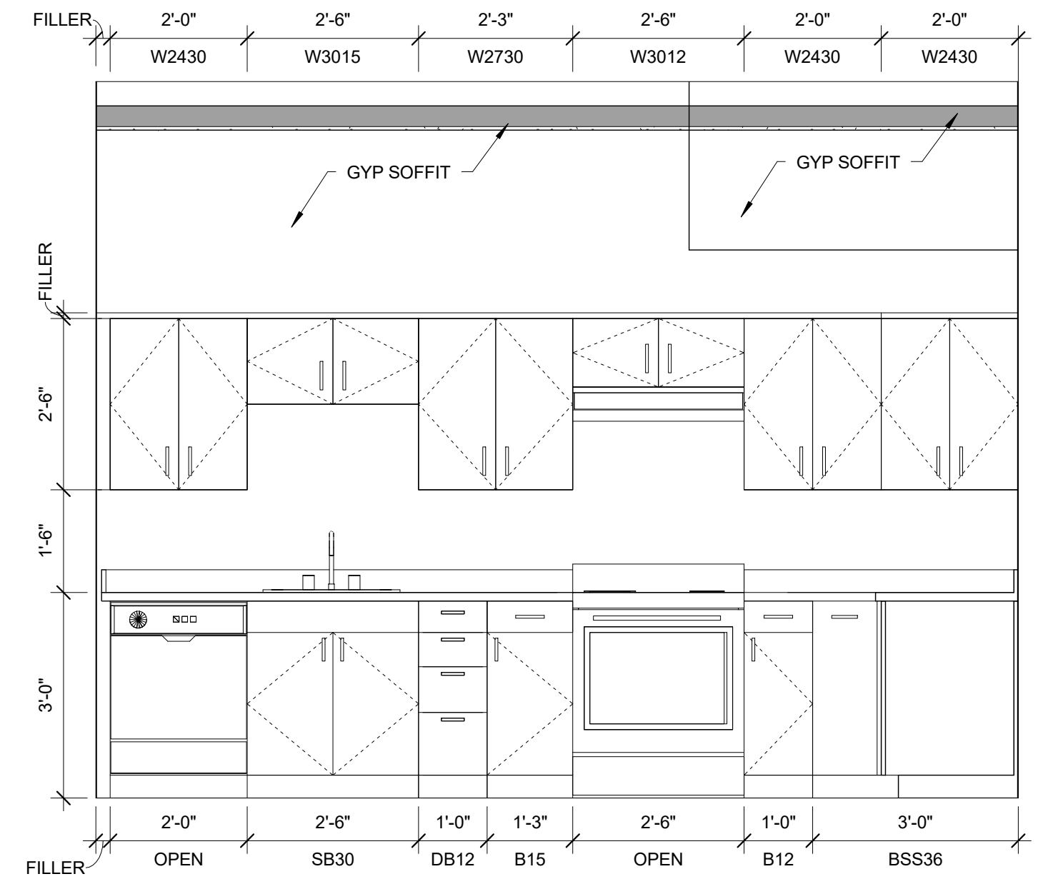
2 | UNIT 119 KITCHEN ELEVATION 1/2" = 1'-0"
