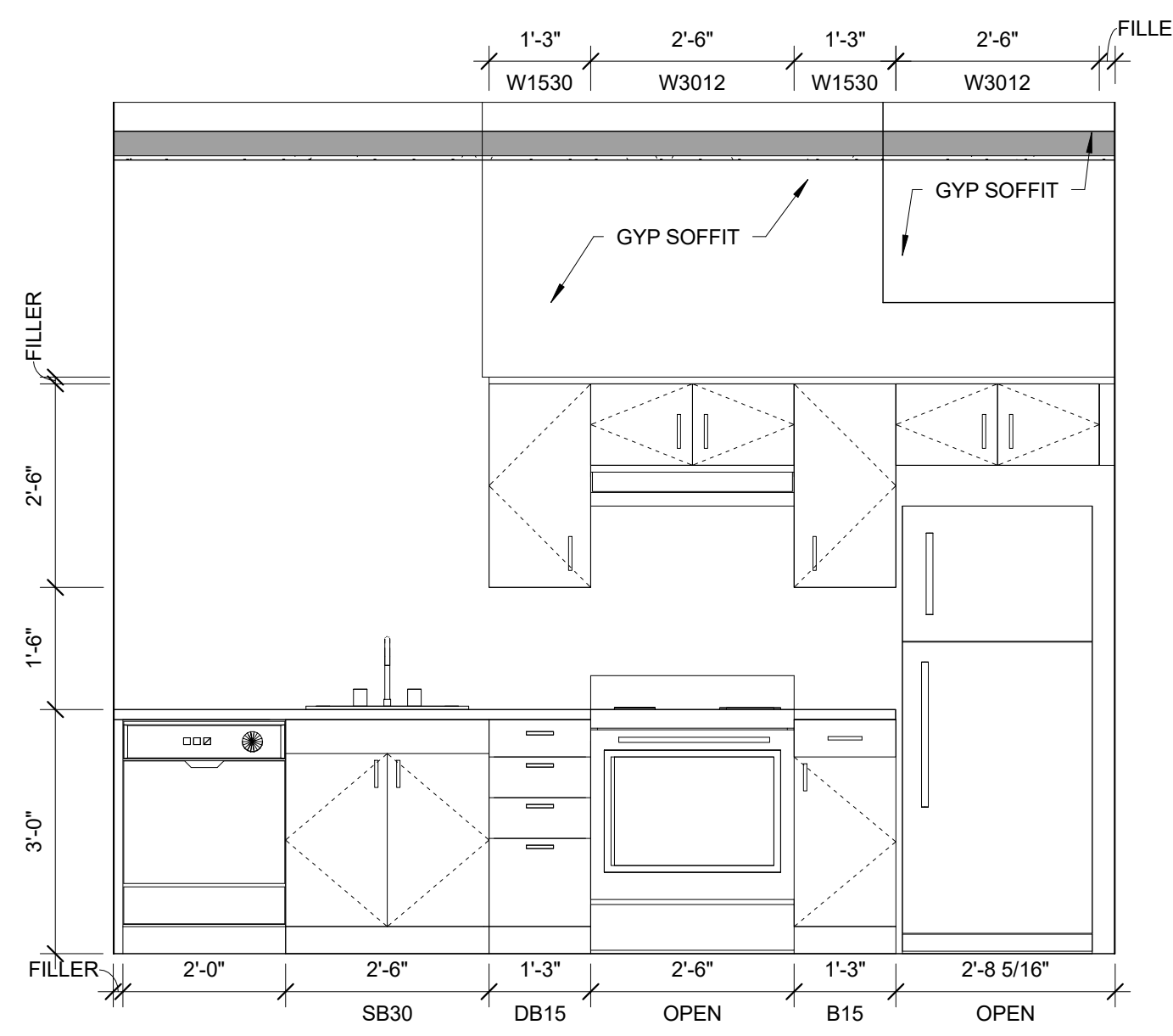
10 | UNIT 117 KITCHEN ELEVATION 1/2" = 1'-0"
