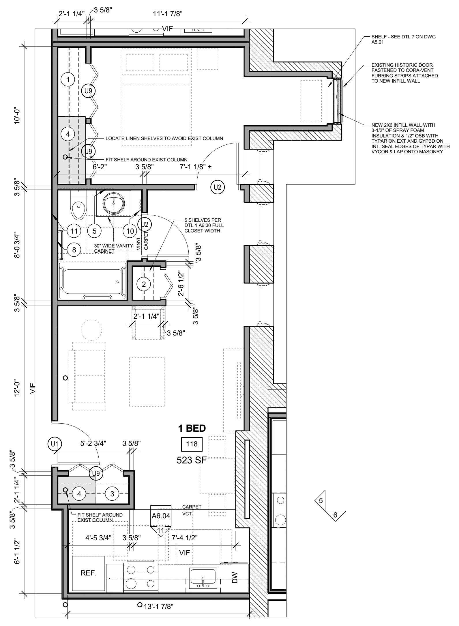
13 | UNIT 118 1/4" = 1'-0" ONE BEDROOM - ANSI 117.1 TYPE B GENERAL STORAGE = 127.0 CU.FT
