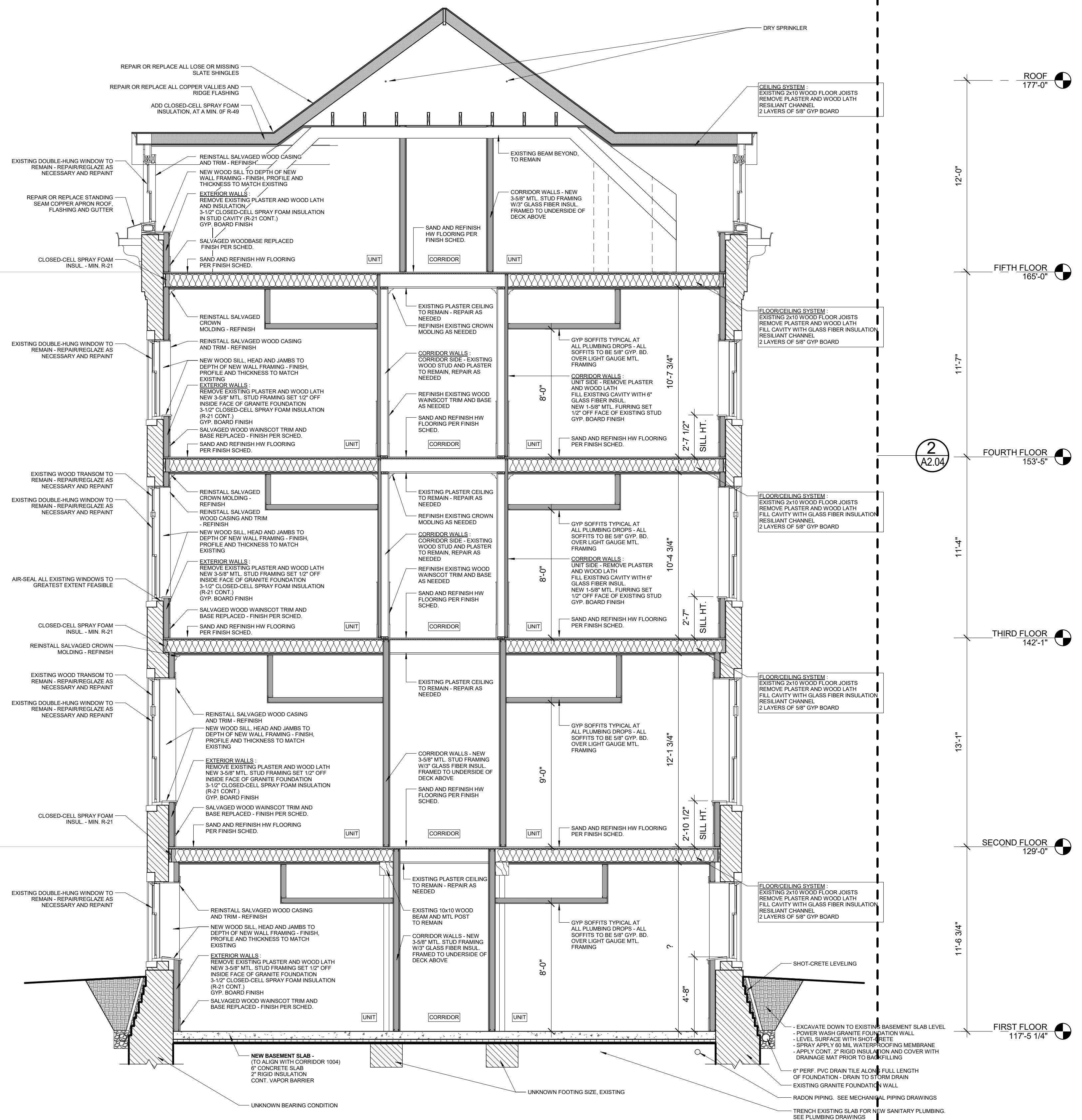
1 | BUILDING SECTION 1/4" = 1'-0"
