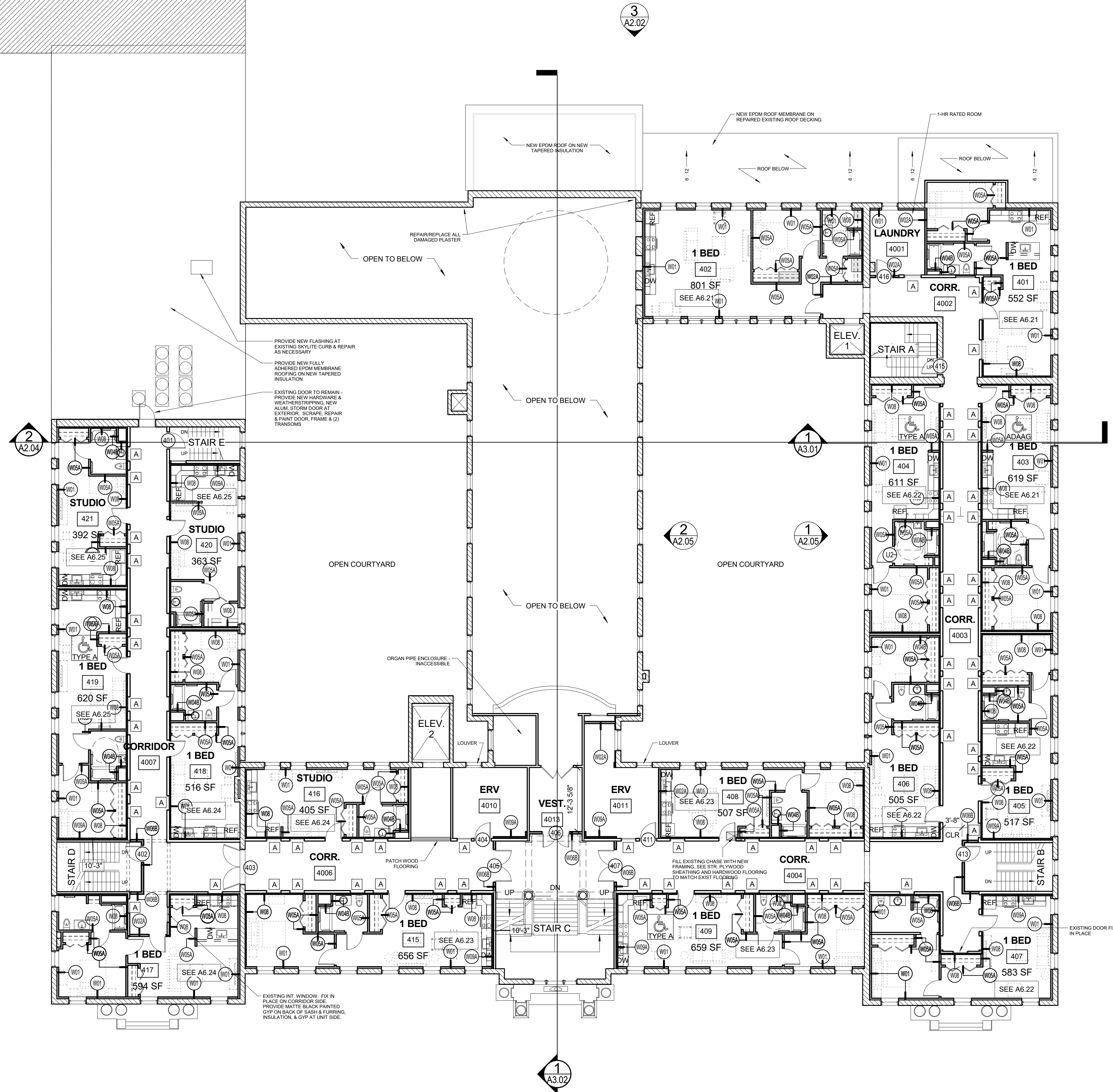
1 | FOURTH FLOOR PLAN 3/32" = 1'-0"
