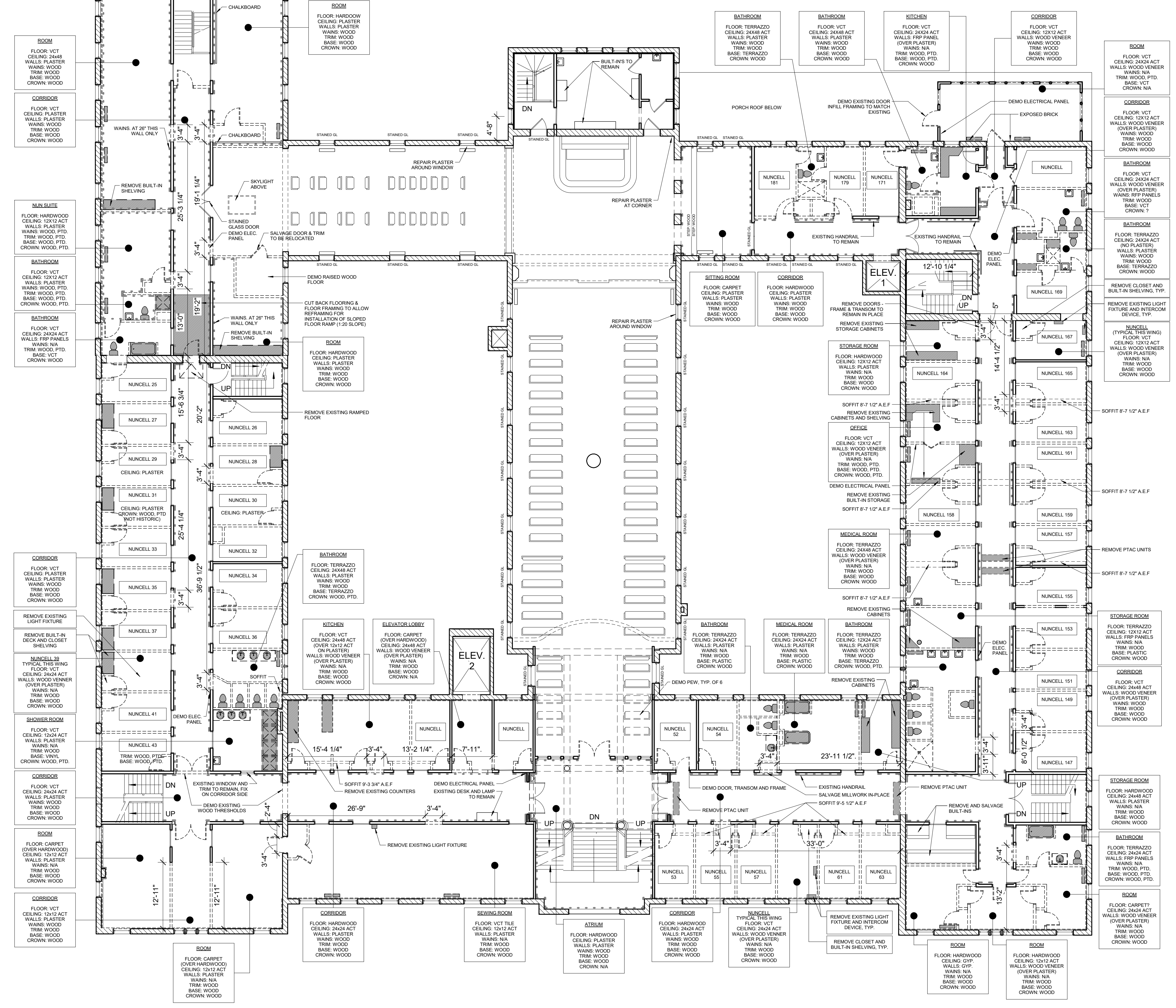
1 | EXISTING THIRD FLOOR PLAN & DEMO 3/32" = 1'-0"
