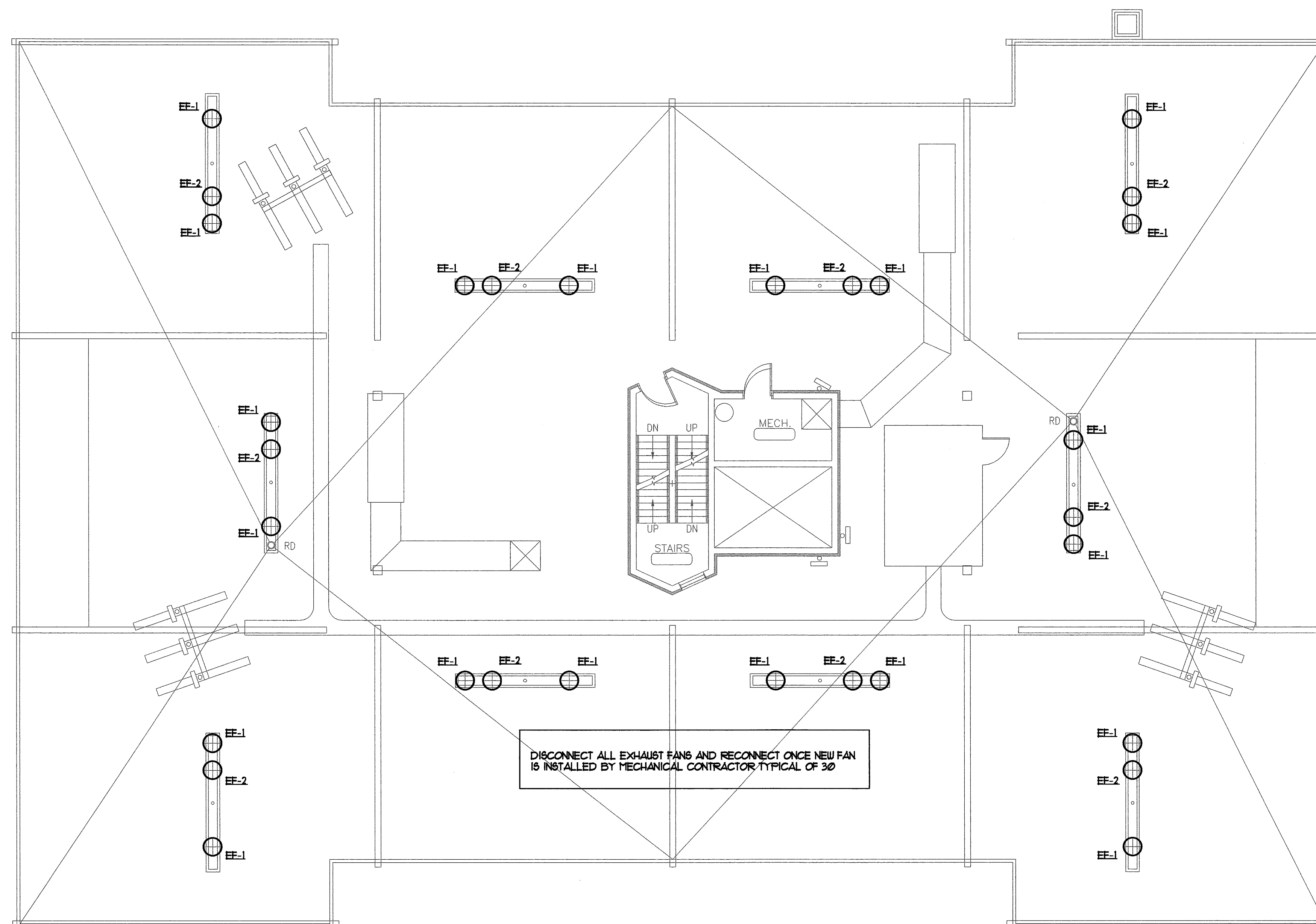
ROOF ELECTRICAL PLAN SCALE - 1/8" = 1'-0"
