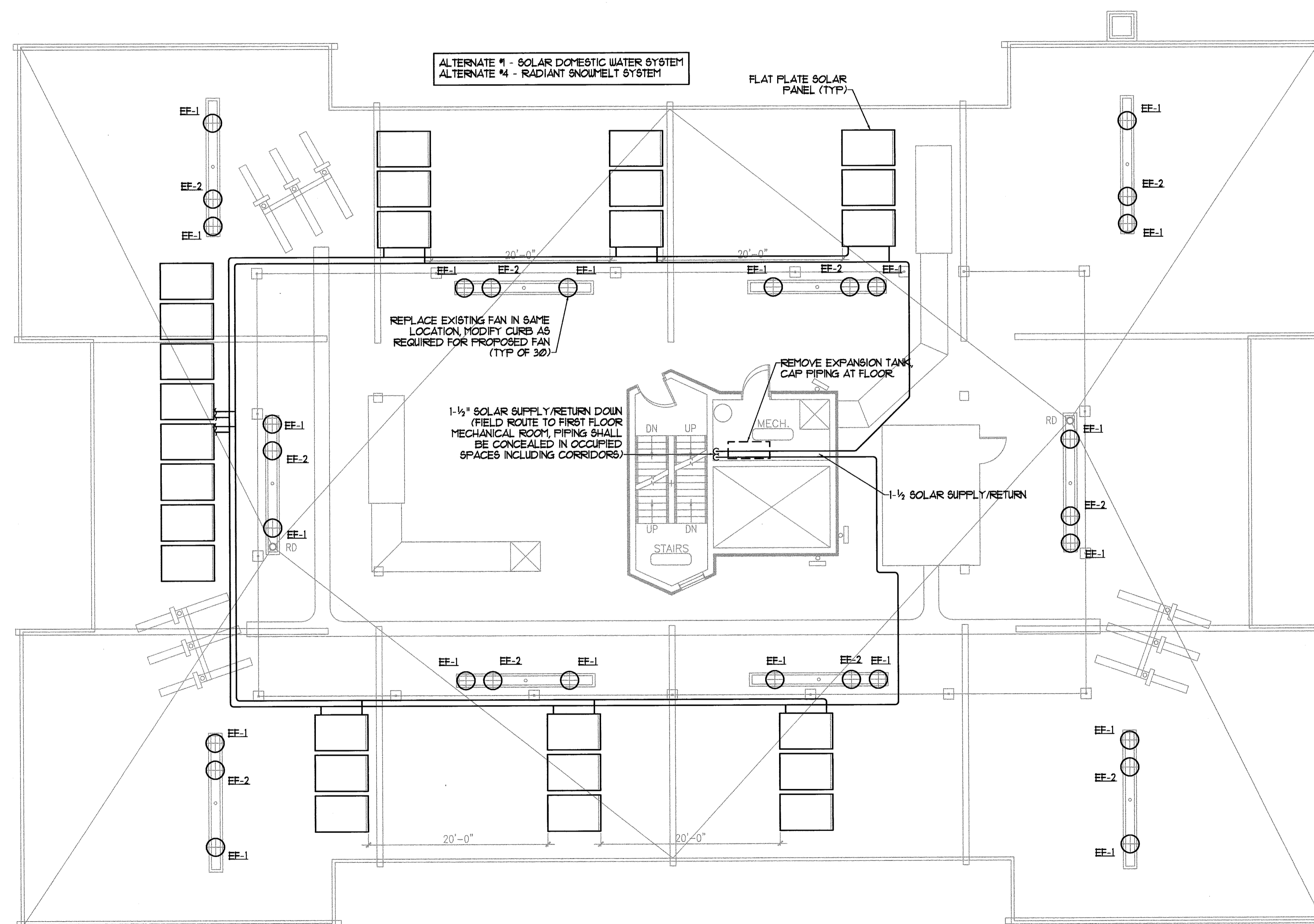
ROOF MECHANICAL PLAN SCALE - 1/8" = 1'-0"
