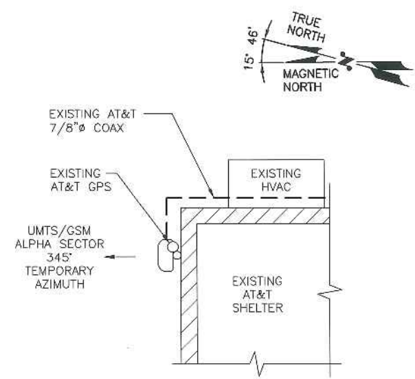
TEMPORARY CONSTRUCTION AZIMUTH (ALPHA SECTOR) SCALE: N.T.S.
