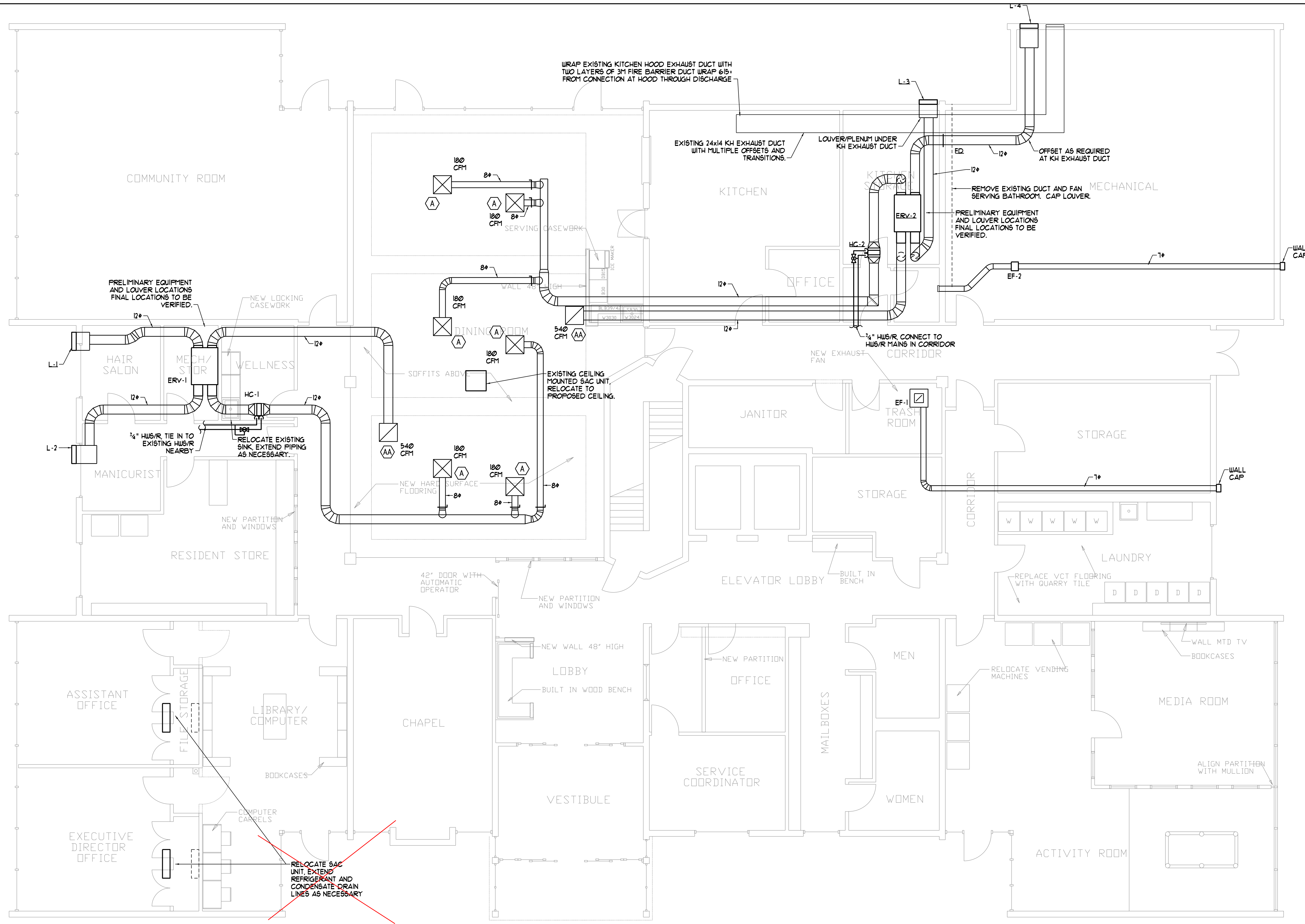
FIRST FLOOR MECHANICAL PLAN SCALE - 3/16" = 1'-0"
