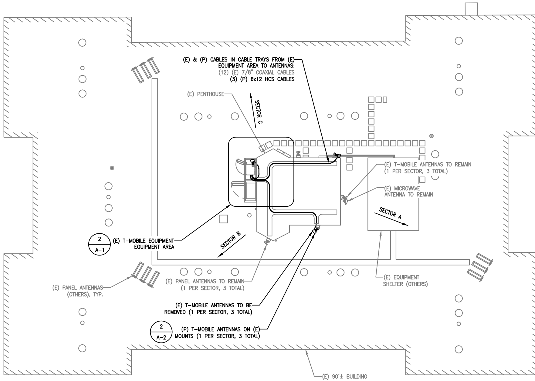
1 COMPOUND PLAN A-1 SCALE: 1/16"=1'-0"
