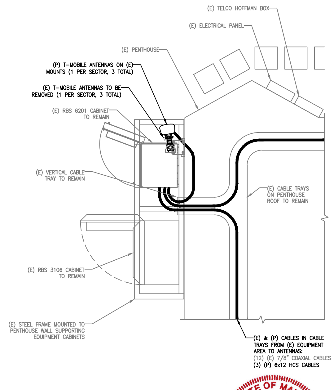
2 EQUIPMENT PLAN A-1 SCALE: 1/4"=1'-0"
