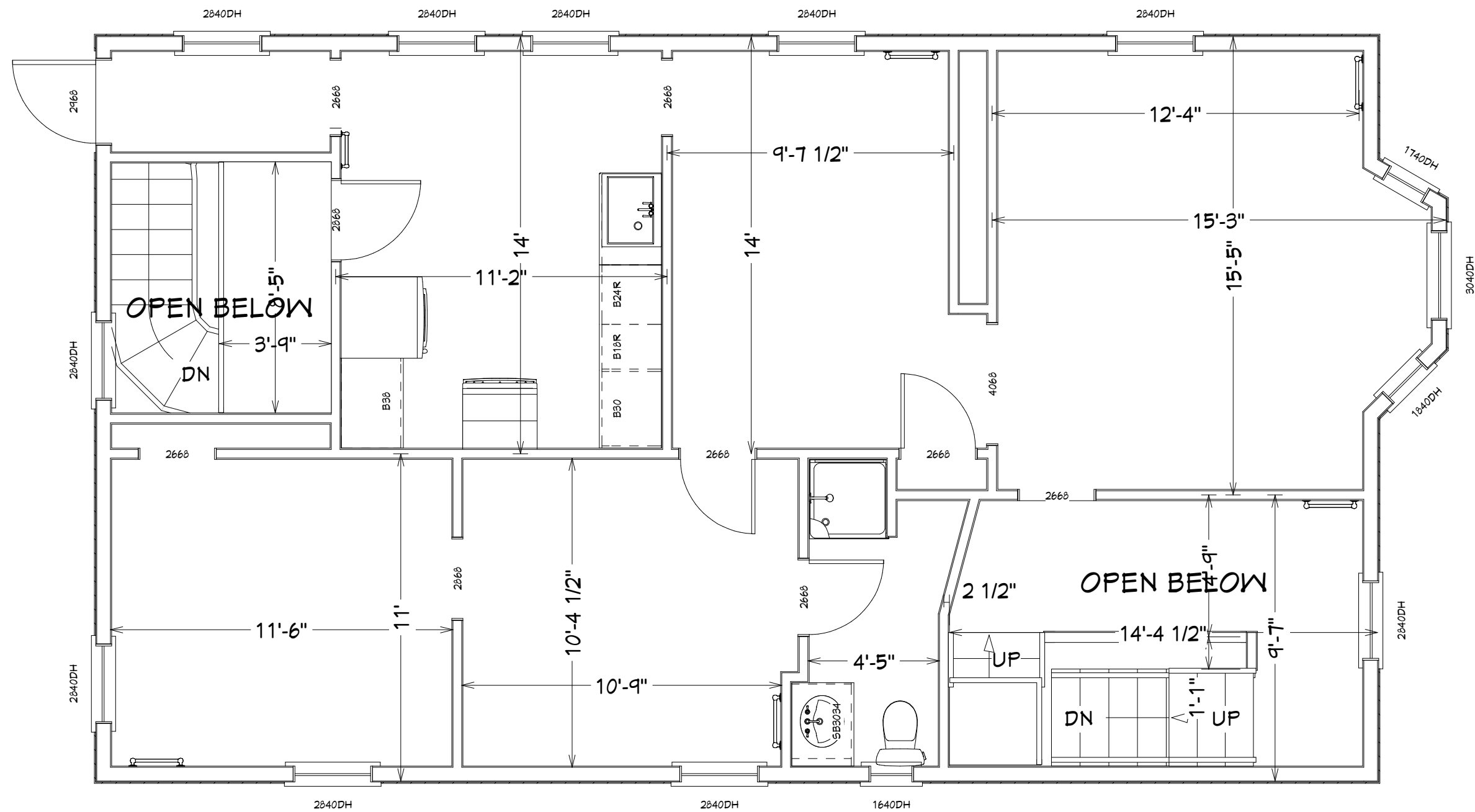
EXISTING SECOND FLOOR PLAN SCALE 1' = 4' - 0"
