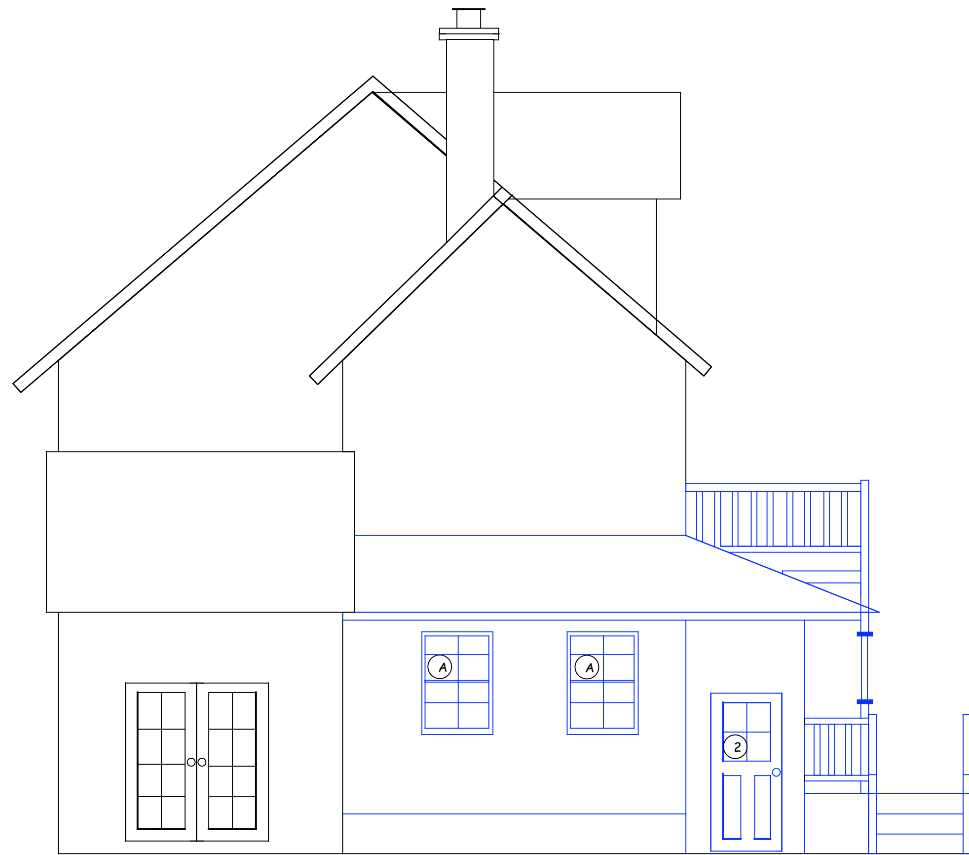
North Elevation
