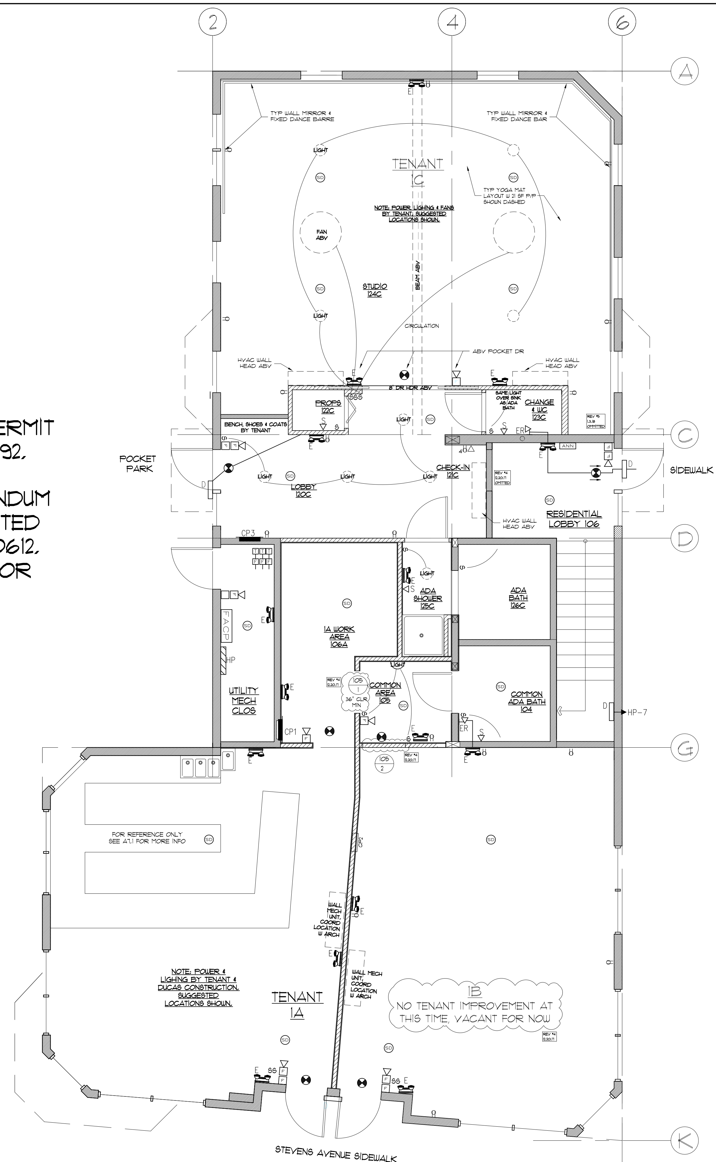
1 1ST FLOOR TENANT IMPROVEMENT LIFE SAFETY, POWER & LIGHTING SCALE = 1/4" = 1'-0"
