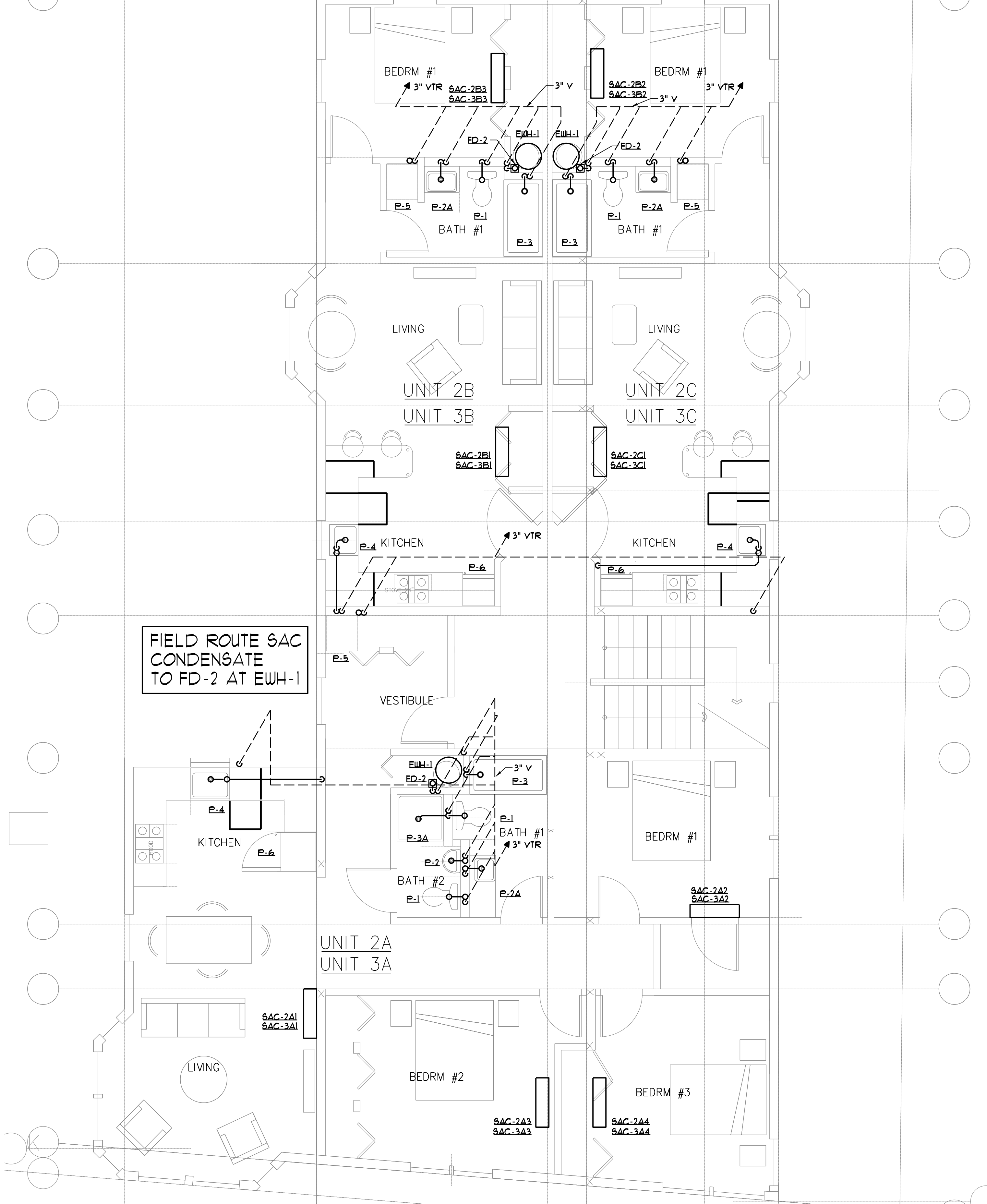
SECOND AND THIRD FLOOR SANITARY PLUMBING PLANS SCALE - 1/4" = 1'-0"
