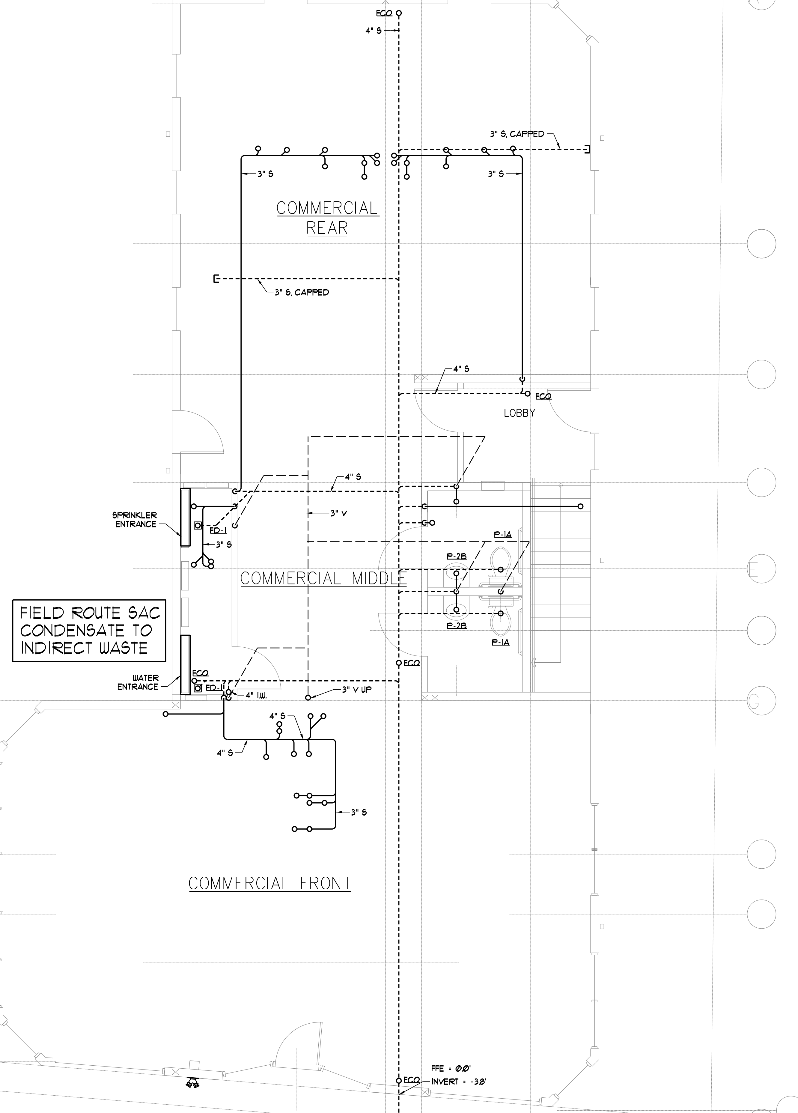
FIRST FLOOR SANITARY PLUMBING PLAN SCALE - 1/4" = 1'-0"
