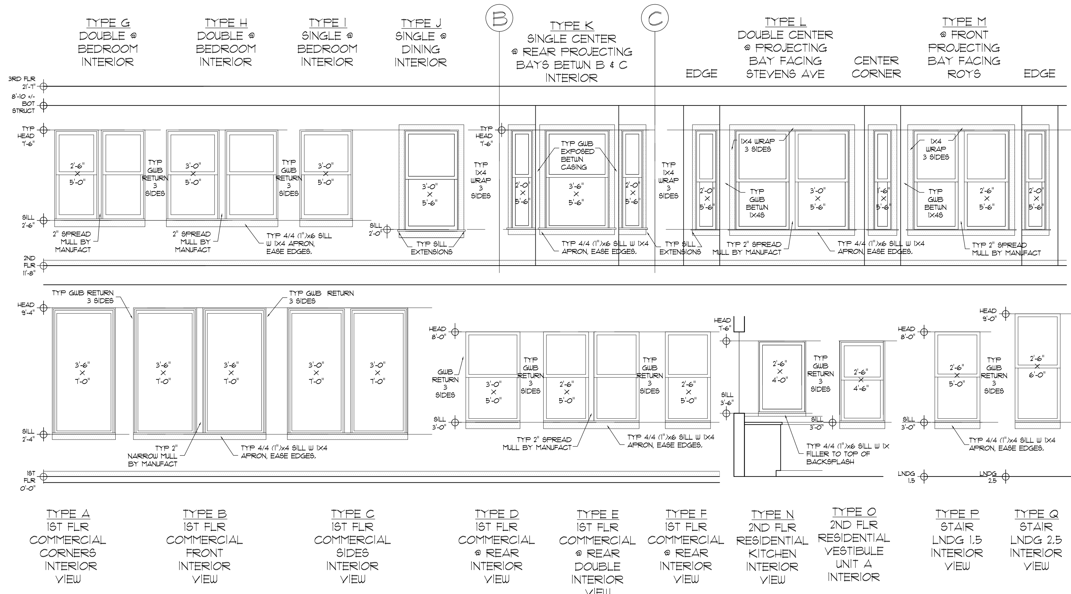
2 WINDOW TYPES INTERIOR VIEW SCALE: NONE
