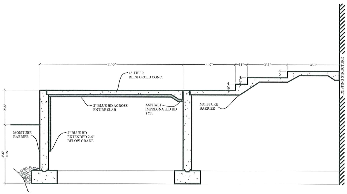
4 FOUNDATION SECTION SCALE: 1/2"=1'
