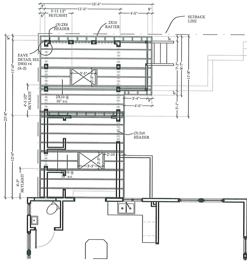
2 FRAMING PLAN SCALE: 1/4"=1'
