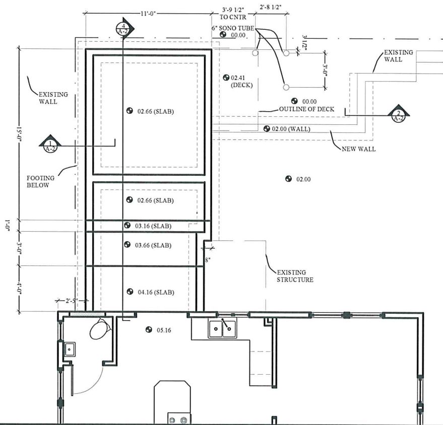
4 FOUNDATION PLAN SCALE: 1/4"=1'
