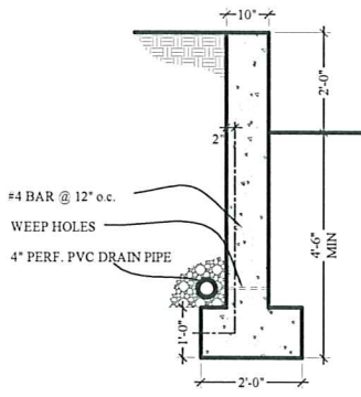
2 RETAINING WALL FOOTING SCALE: 1/2"=1'
