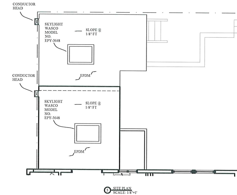
5 SITE PLAN SCALE: 1/8"=1'
