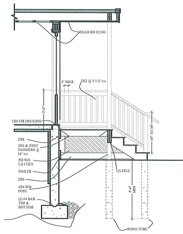
3 DECK SECTION SCALE: 1/2"=1'
