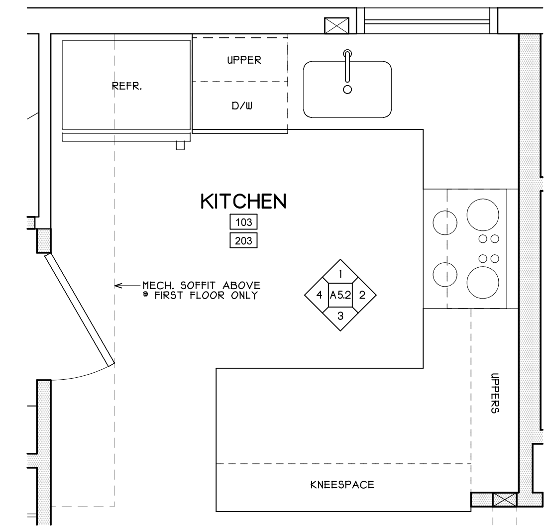
A KITCHEN PLAN - TYP. BOTH FLOORS A5.2 SCALE: 1/2"=1'-0"
