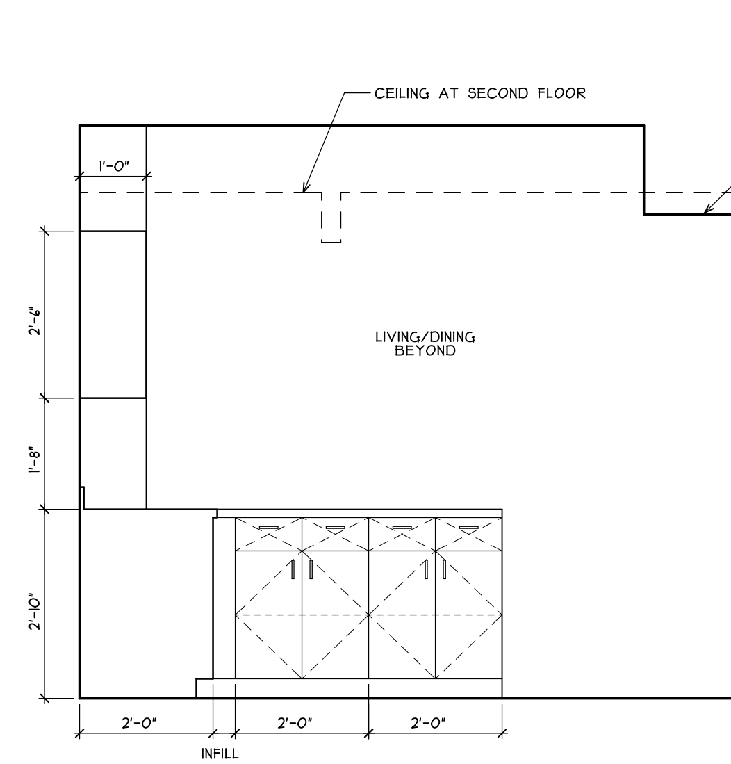
3 KITCHEN, TYPICAL A5.2 SCALE: 1/2"=1'-0"
