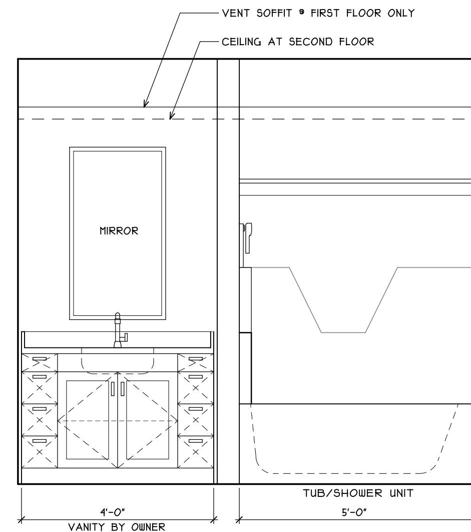
6 BATH, TYPICAL A5.2 SCALE: 1/2"=1'-0"
