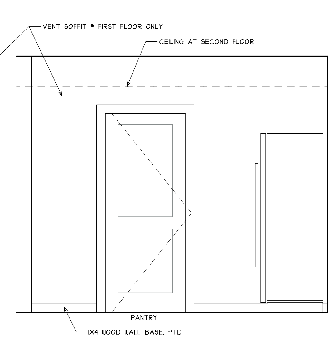
4 KITCHEN, TYPICAL A5.2 SCALE: 1/2"=1'-0"
