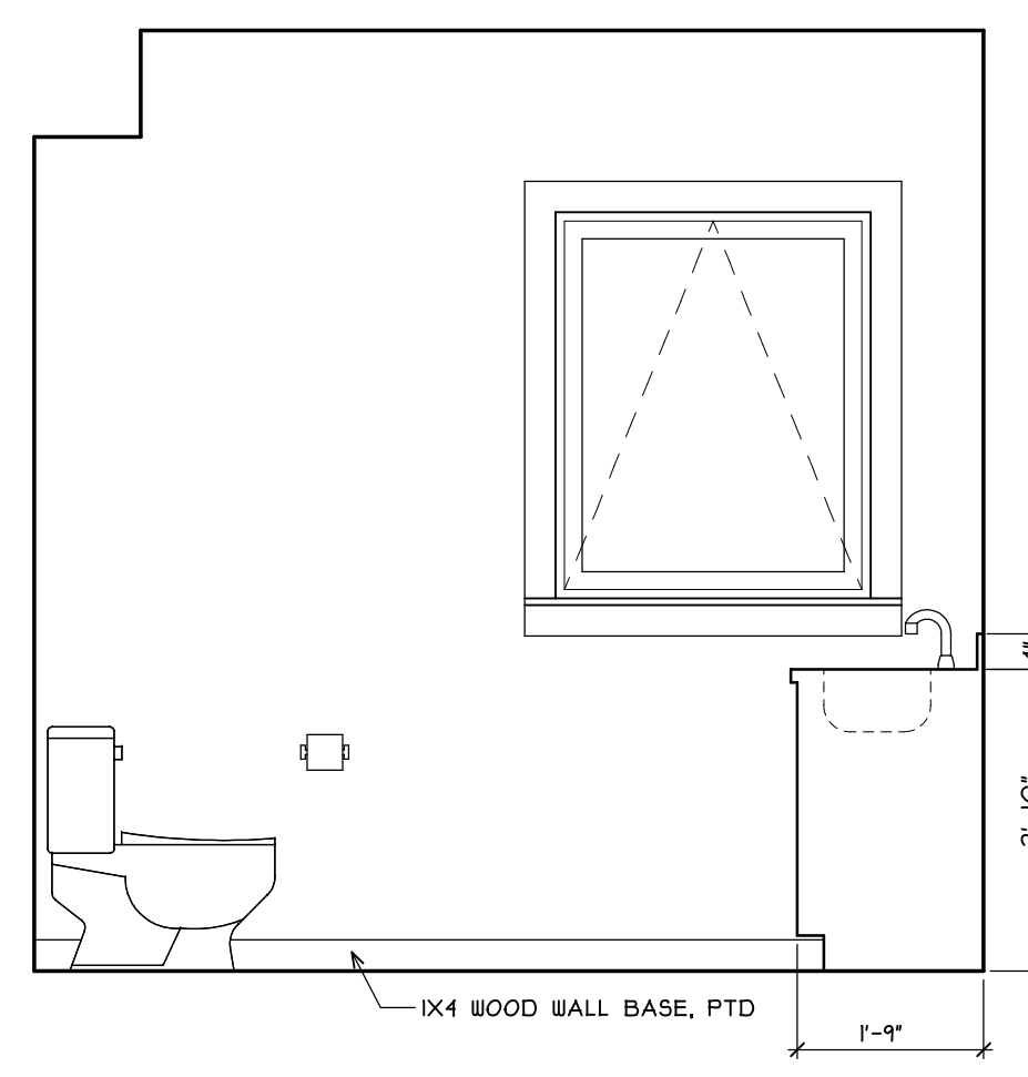
5A BATH - FIRST FLOOR A5.2 SCALE: 1/2"=1'-0"
