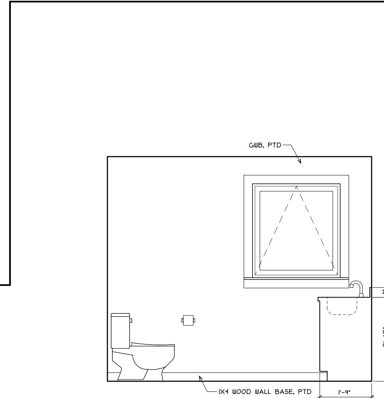
5B BATH - SECOND FLOOR A5.2 SCALE: 1/2"=1'-0"
