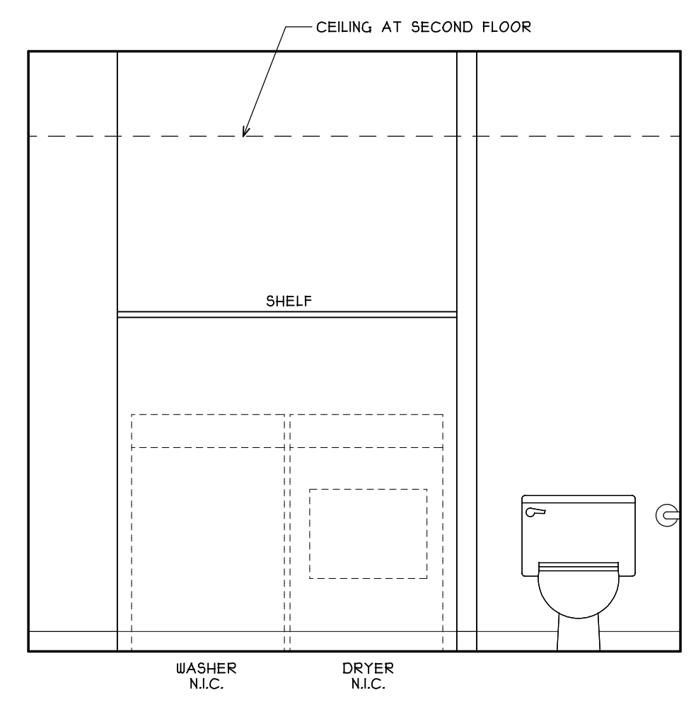
8 BATH - FIRST FLOOR A5.2 SCALE: 1/2"=1'-0"
