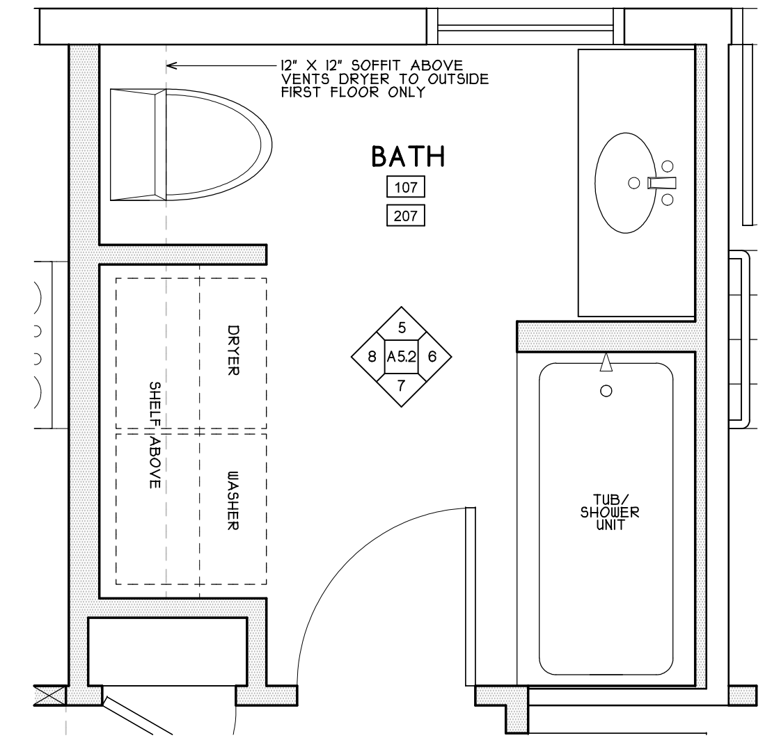
B BATH PLAN - TYP. BOTH FLOORS A5.2 SCALE: 1/2"=1'-0"
