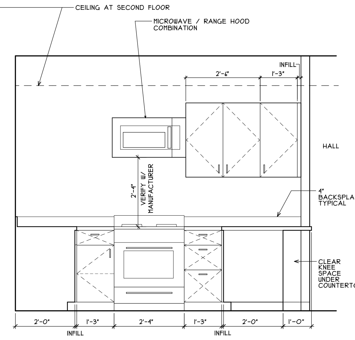
2 KITCHEN, TYPICAL A5.2 SCALE: 1/2"=1'-0"
