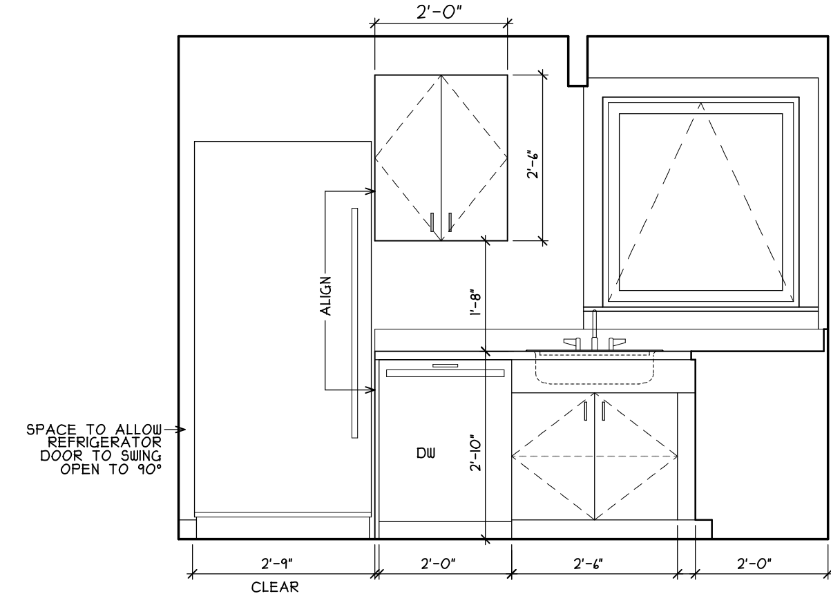
1B KITCHEN - SECOND FLOOR A5.2 SCALE: 1/2"=1'-0"
