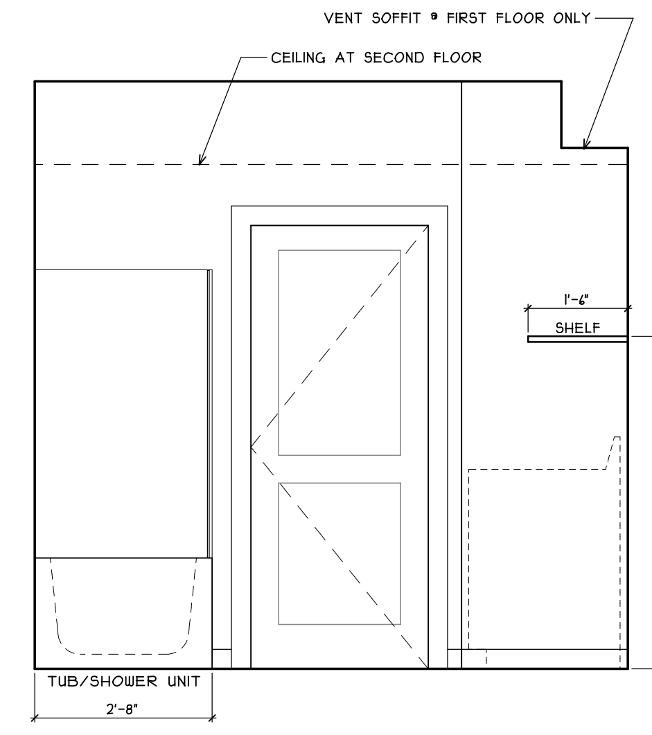
7 BATH - FIRST FLOOR A5.2 SCALE: 1/2"=1'-0"
