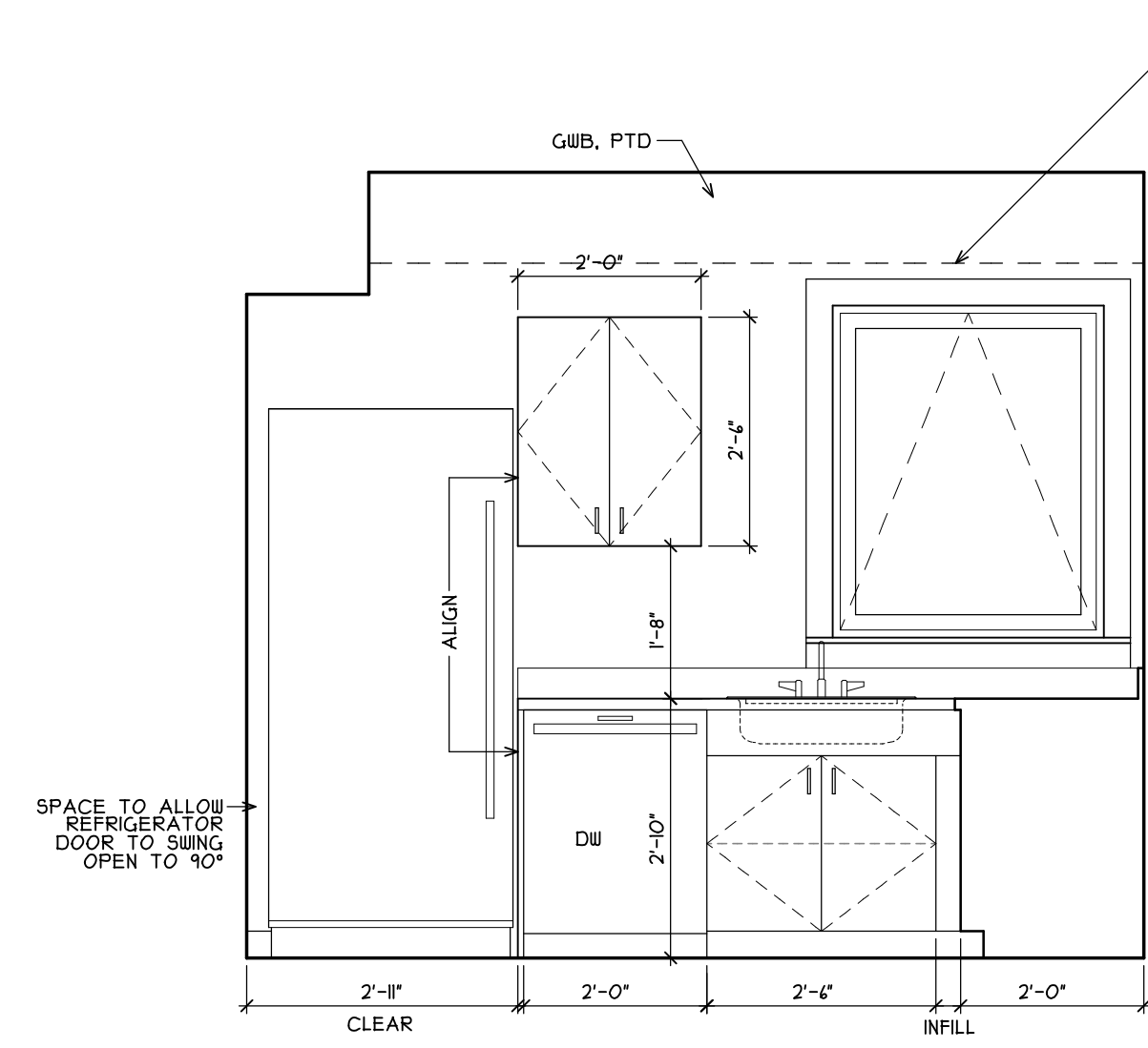
1A KITCHEN - FIRST FLOOR A5.2 SCALE: 1/2"=1'-0"
