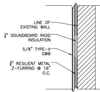
WALL TYPE 2
