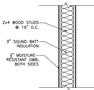
WALL TYPE 1
