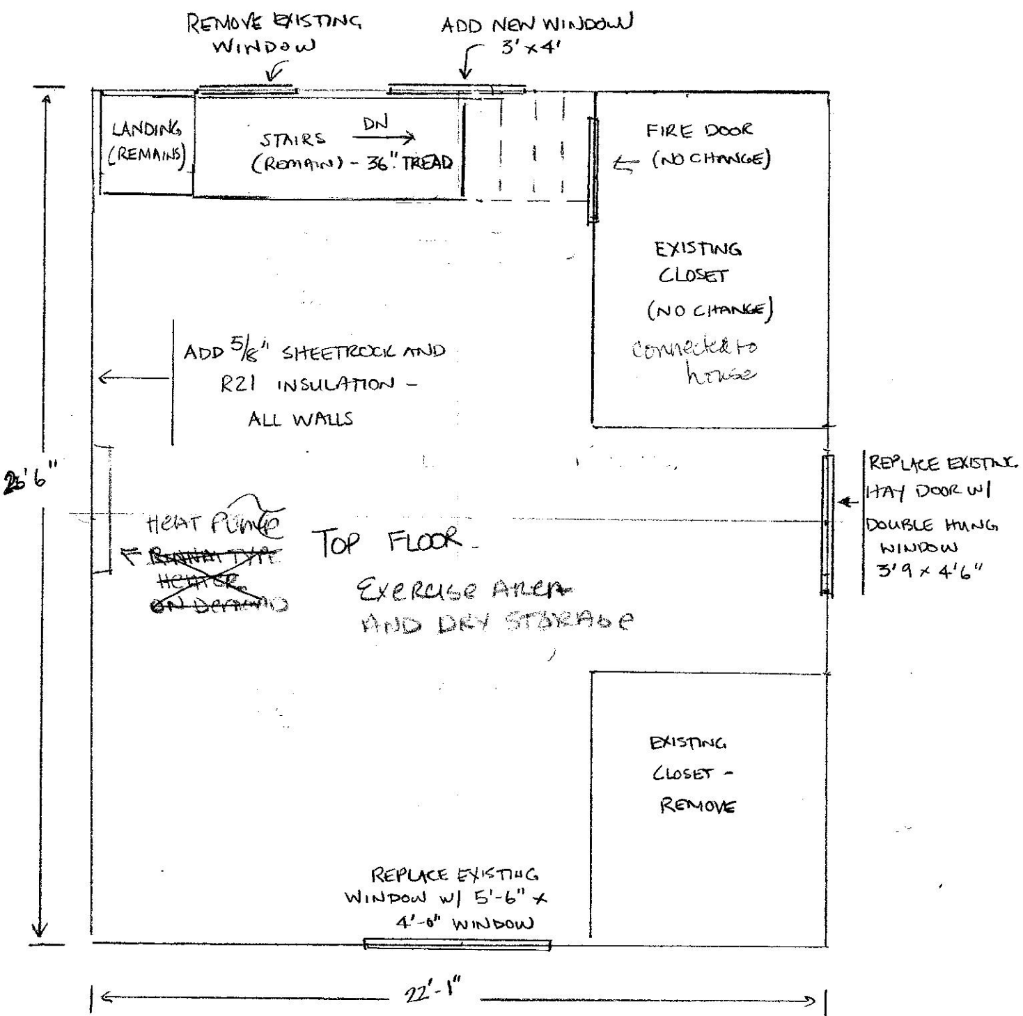
PLAN VIEW - TOP FLOOR
