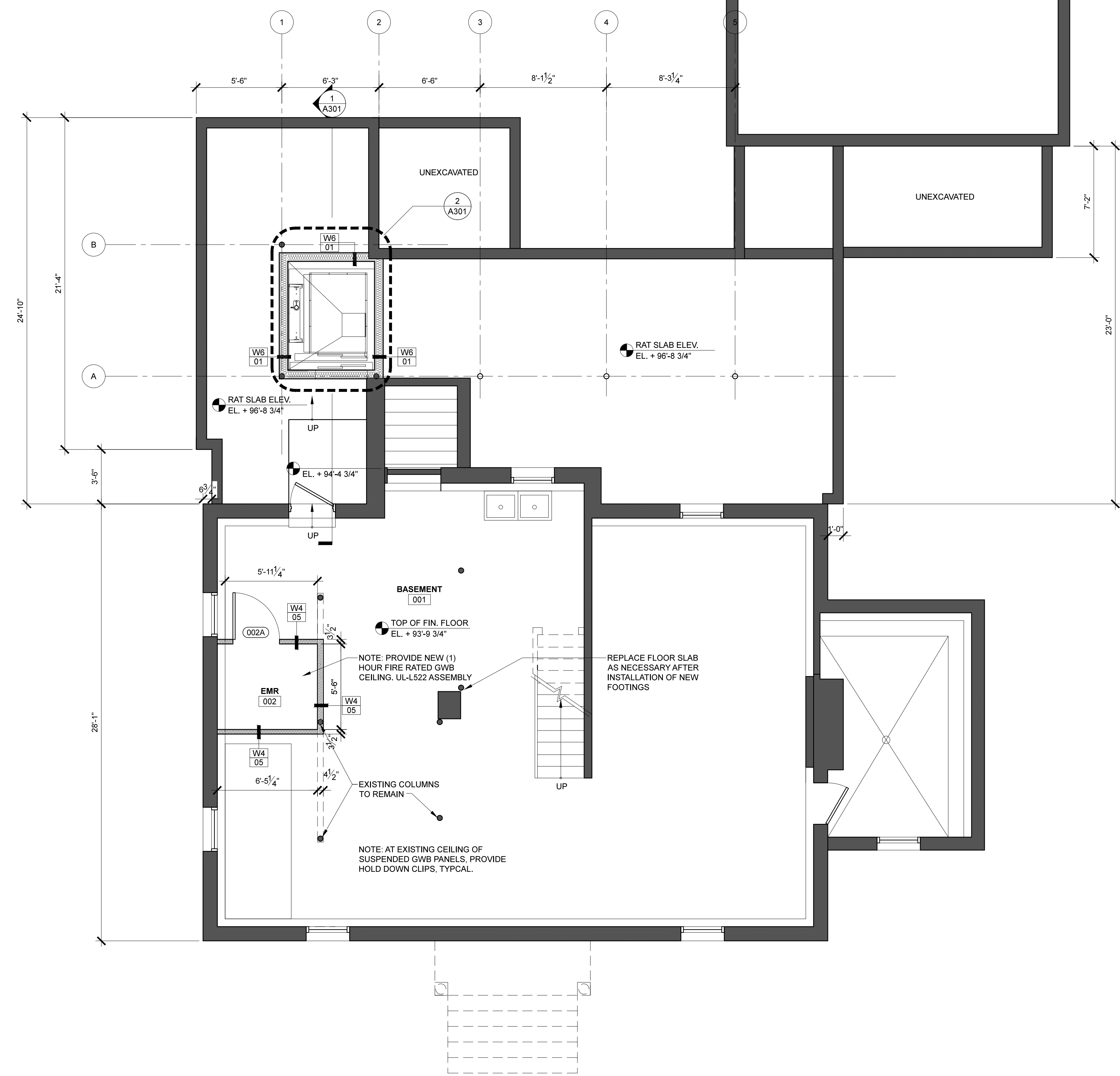
1 Basement Plan SCALE: 1/4" = 1'-0"
