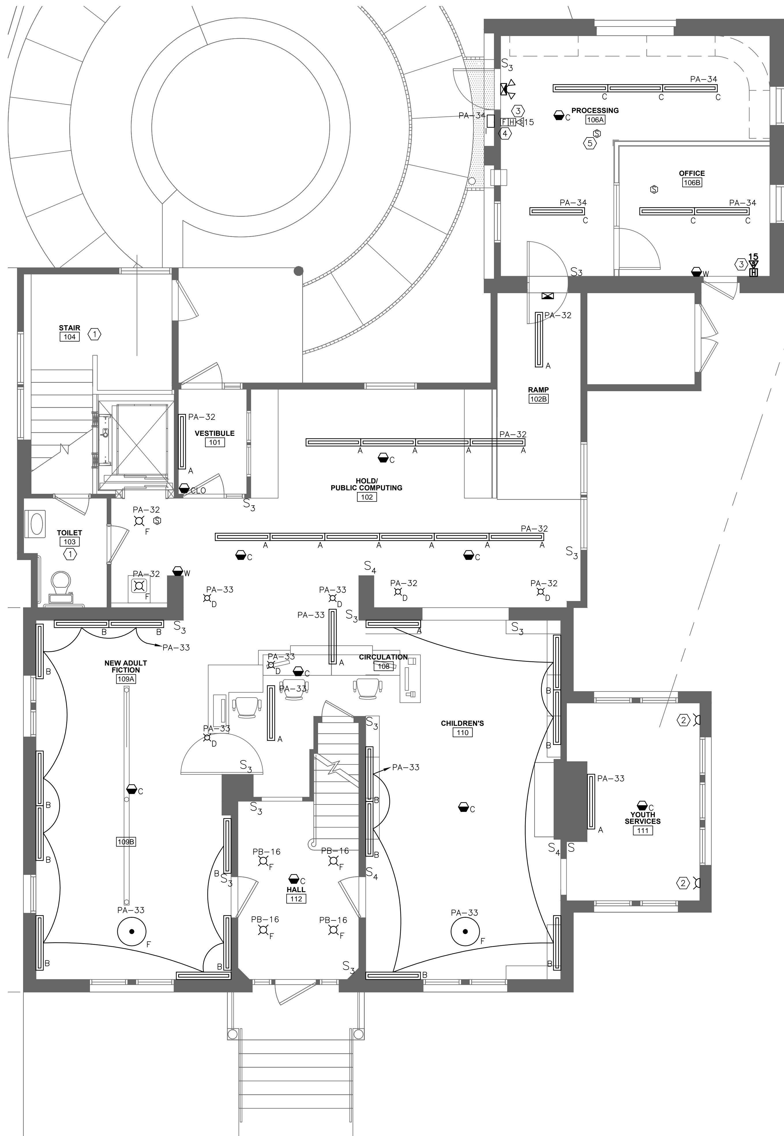
1 ELECTRICAL LIGHTING & FIRE ALARM PLAN - FIRST FLOOR SCALE: 1/4"=1'
