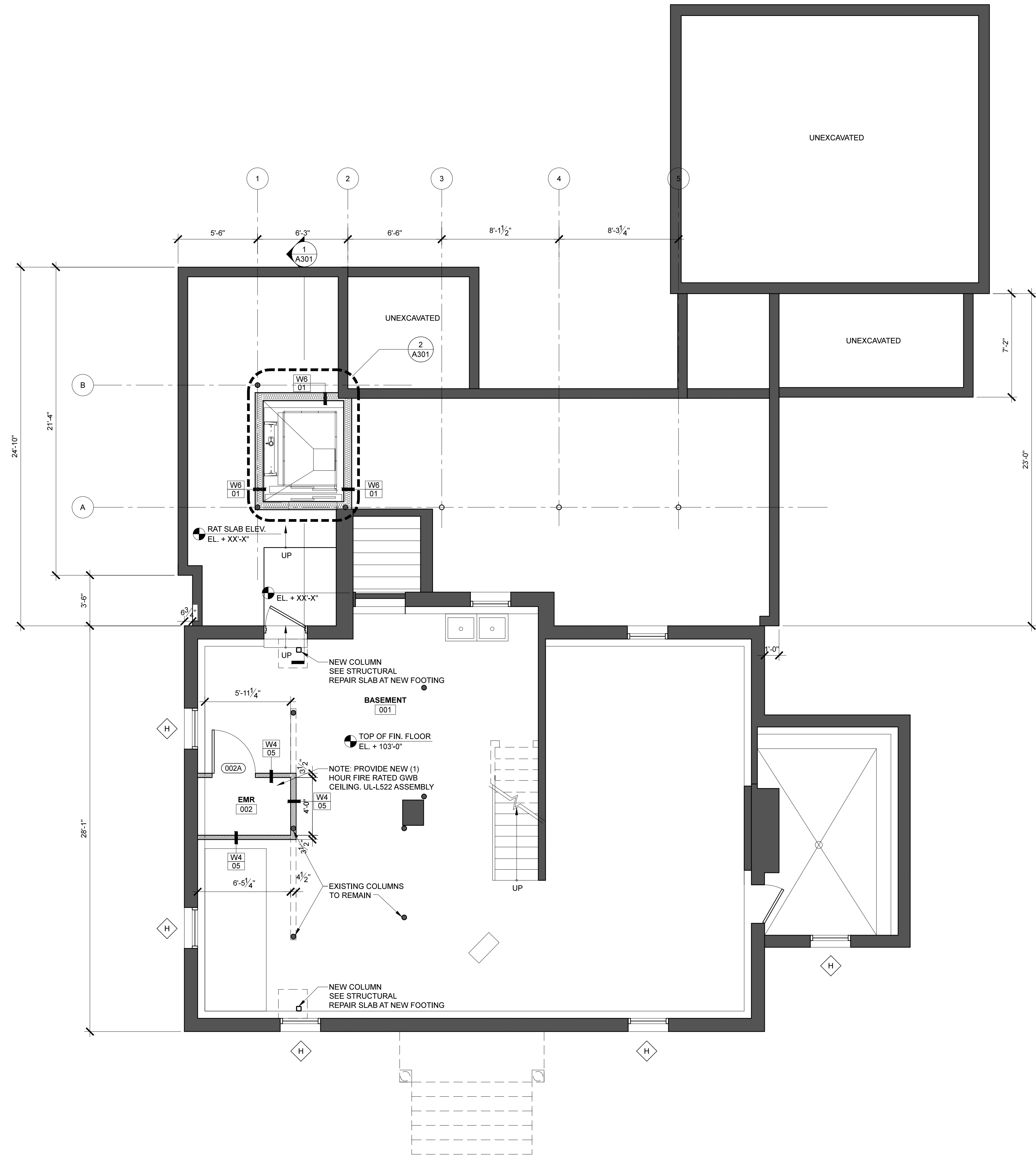
1 Basement Plan SCALE: 1/4" = 1'-0"
