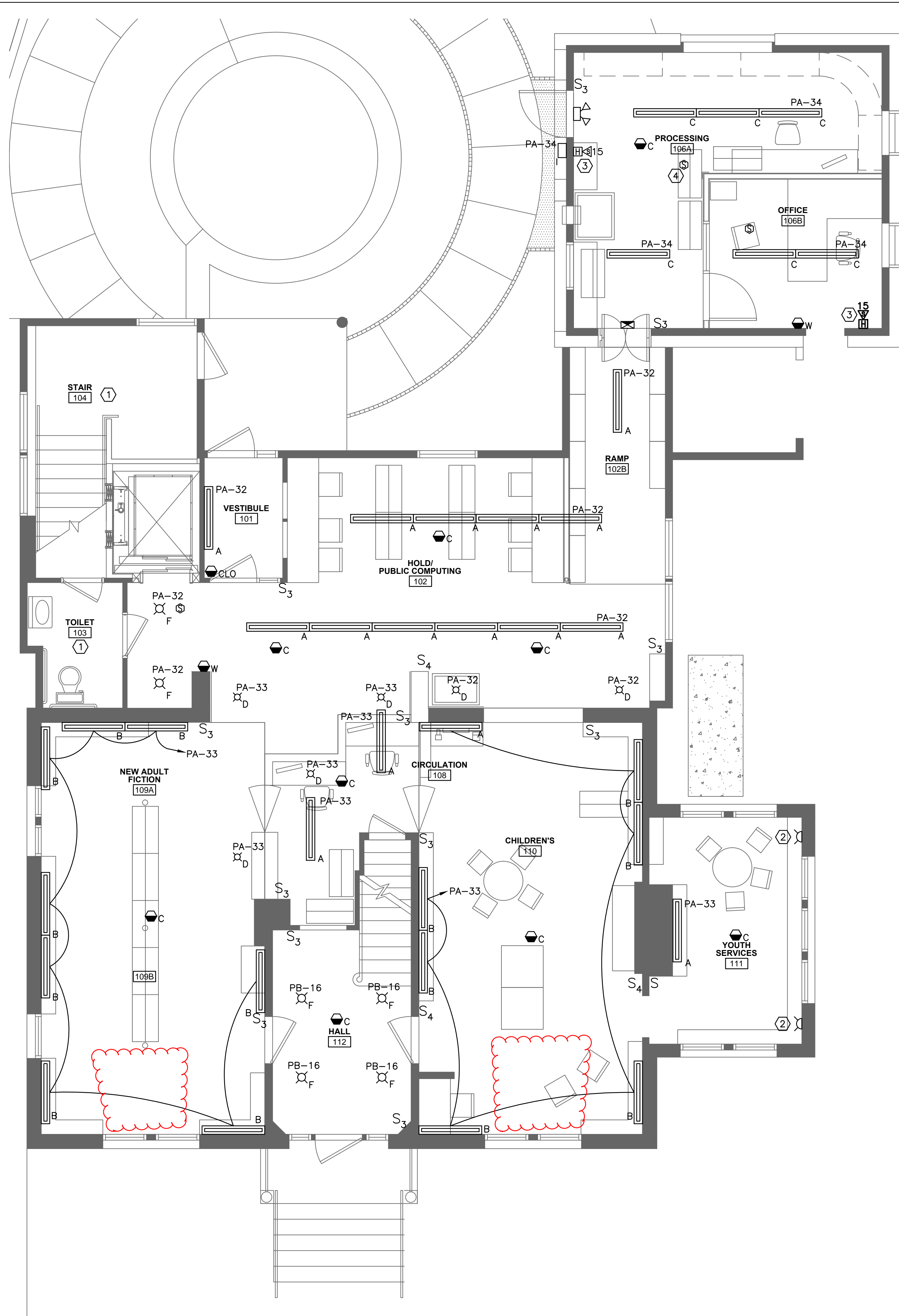
1 ELECTRICAL LIGHTING & FIRE ALARM PLAN - FIRST FLOOR SCALE: 1/4"=1'
