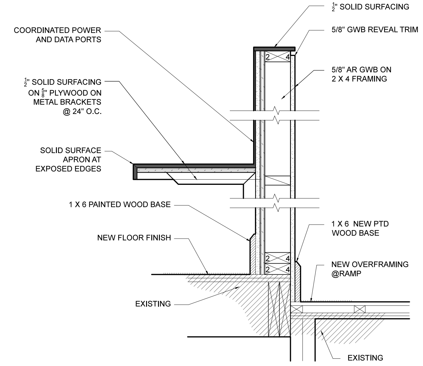
4 Counter Section SCALE: 1 1/2" = 1'-0"
