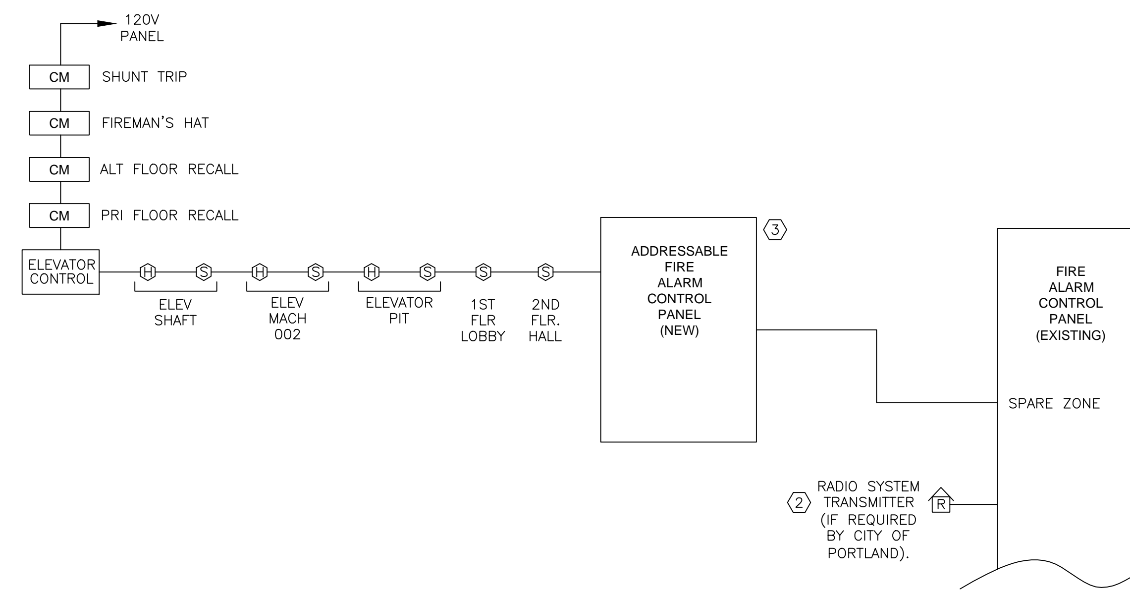
2 FIRE ALARM RISER DIAGRAM – NEW AND EXISTING(PARTIAL) SCALE: NOT TO SCALE
