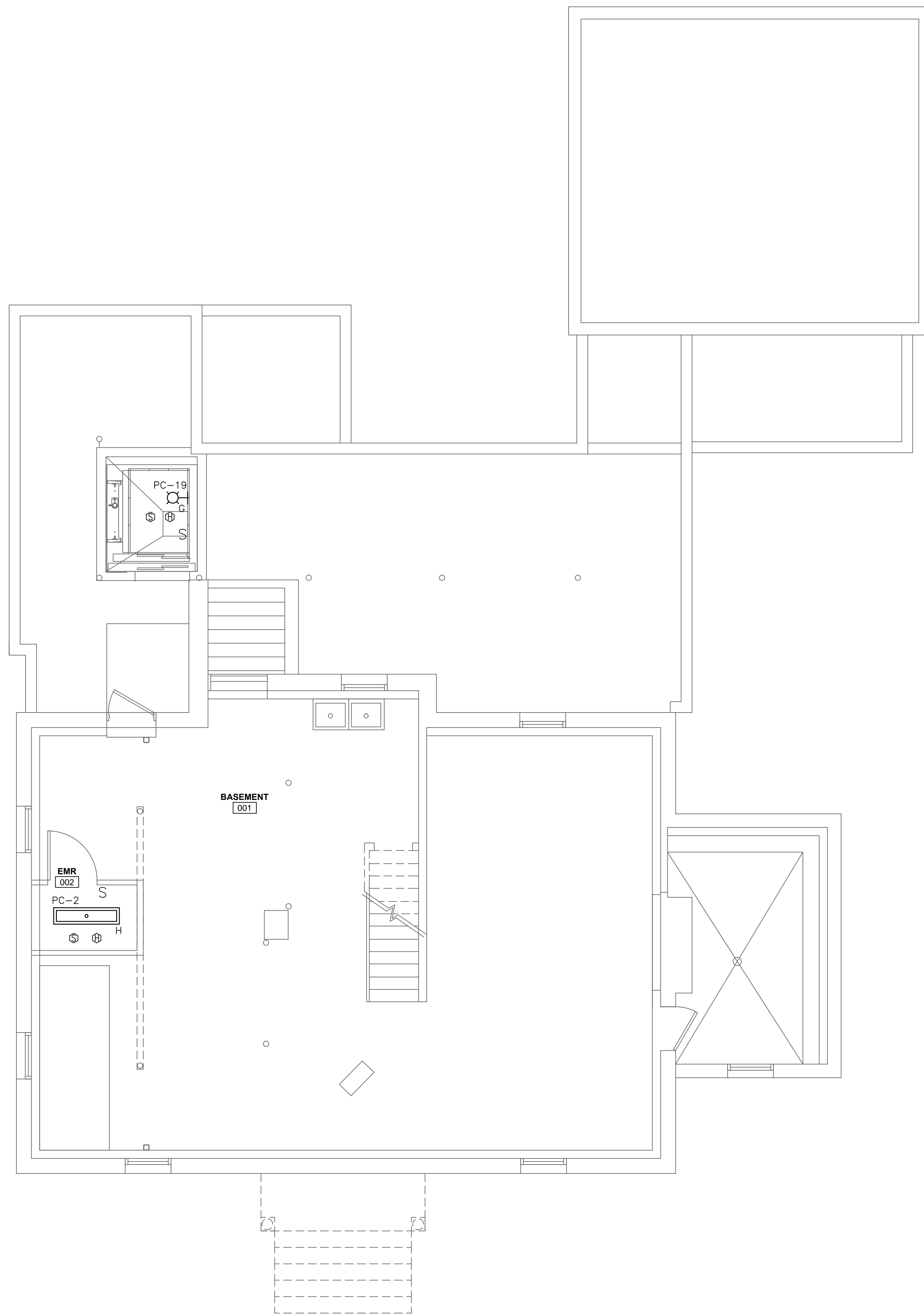
1 ELECTRICAL LIGHTING & FIRE ALARM PLAN – BASEMENT SCALE: 1/4"=1'
