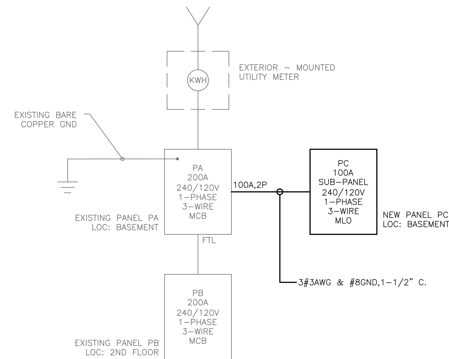
3 ONE LINE DIAGRAM (BASE BID) SCALE: NOT TO SCALE
