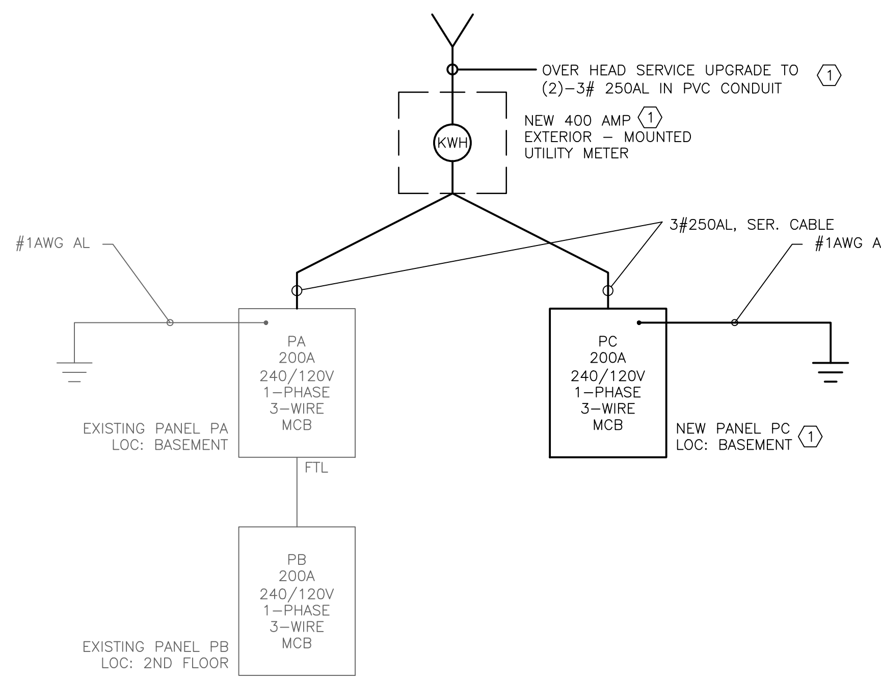
2 ONE LINE DIAGRAM (ADD ALTERNATE) SCALE: NOT TO SCALE
