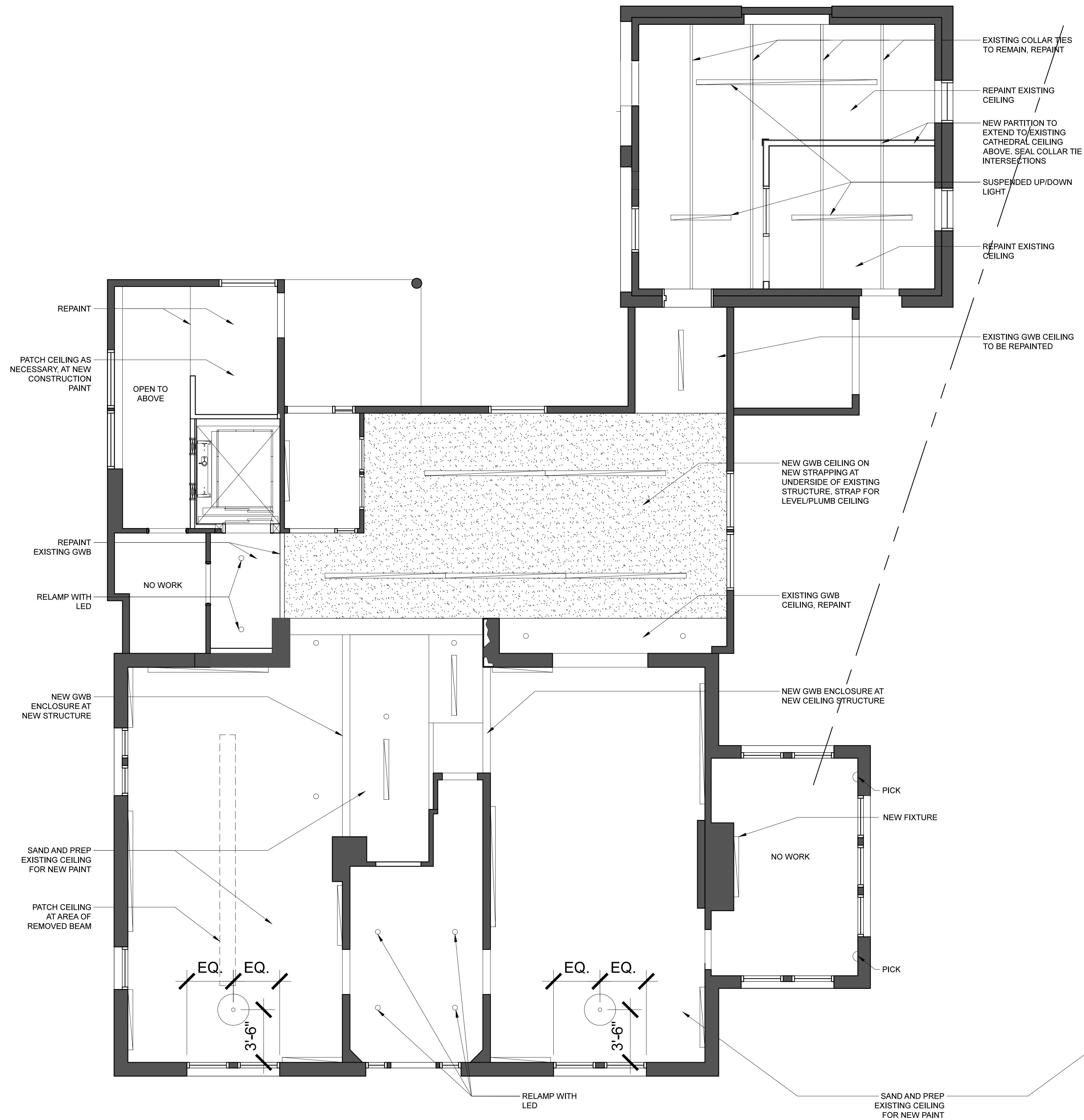
1 First Floor Reflected Ceiling Plan SCALE: 1/8" = 1'-0"
