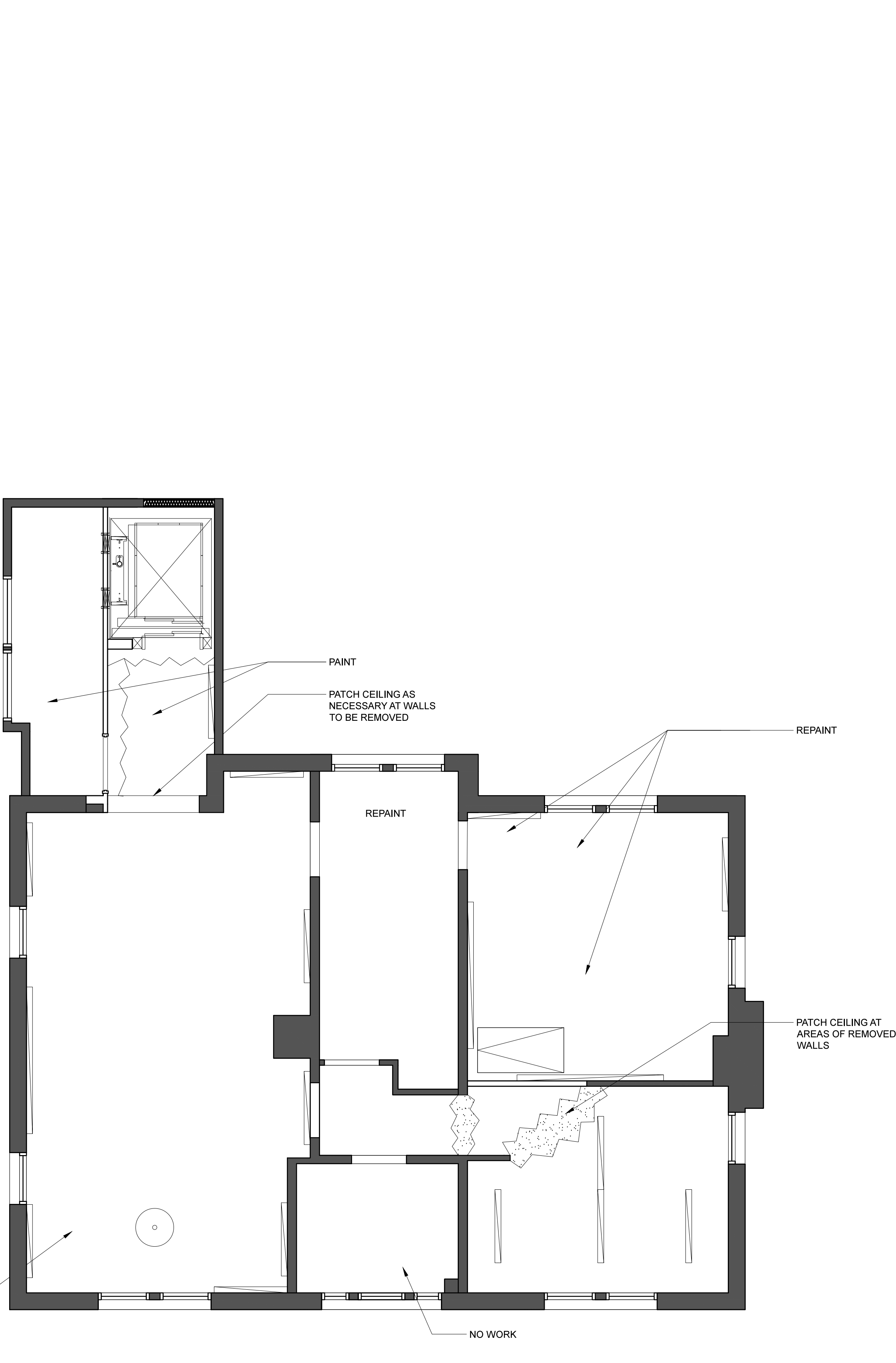
2 Second Floor Reflected Ceiling Plan SCALE: 1/8" = 1'-0"
