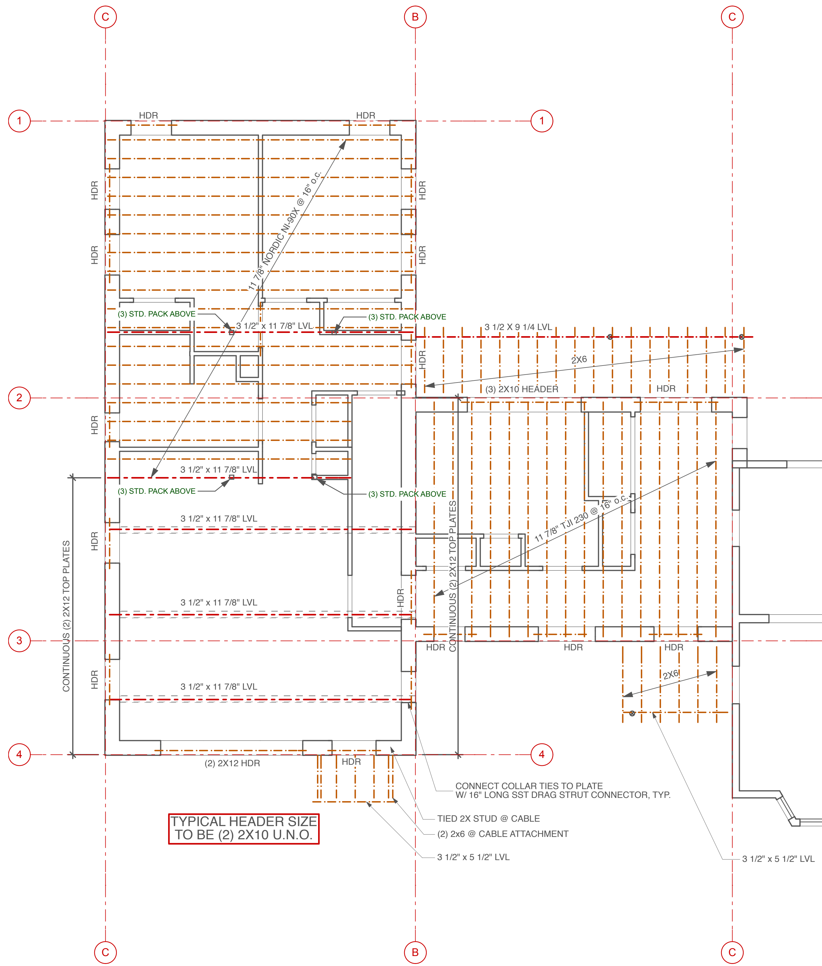
2 2ND FLOOR FRAMING SCALE: 1/4" = 1'-0"
