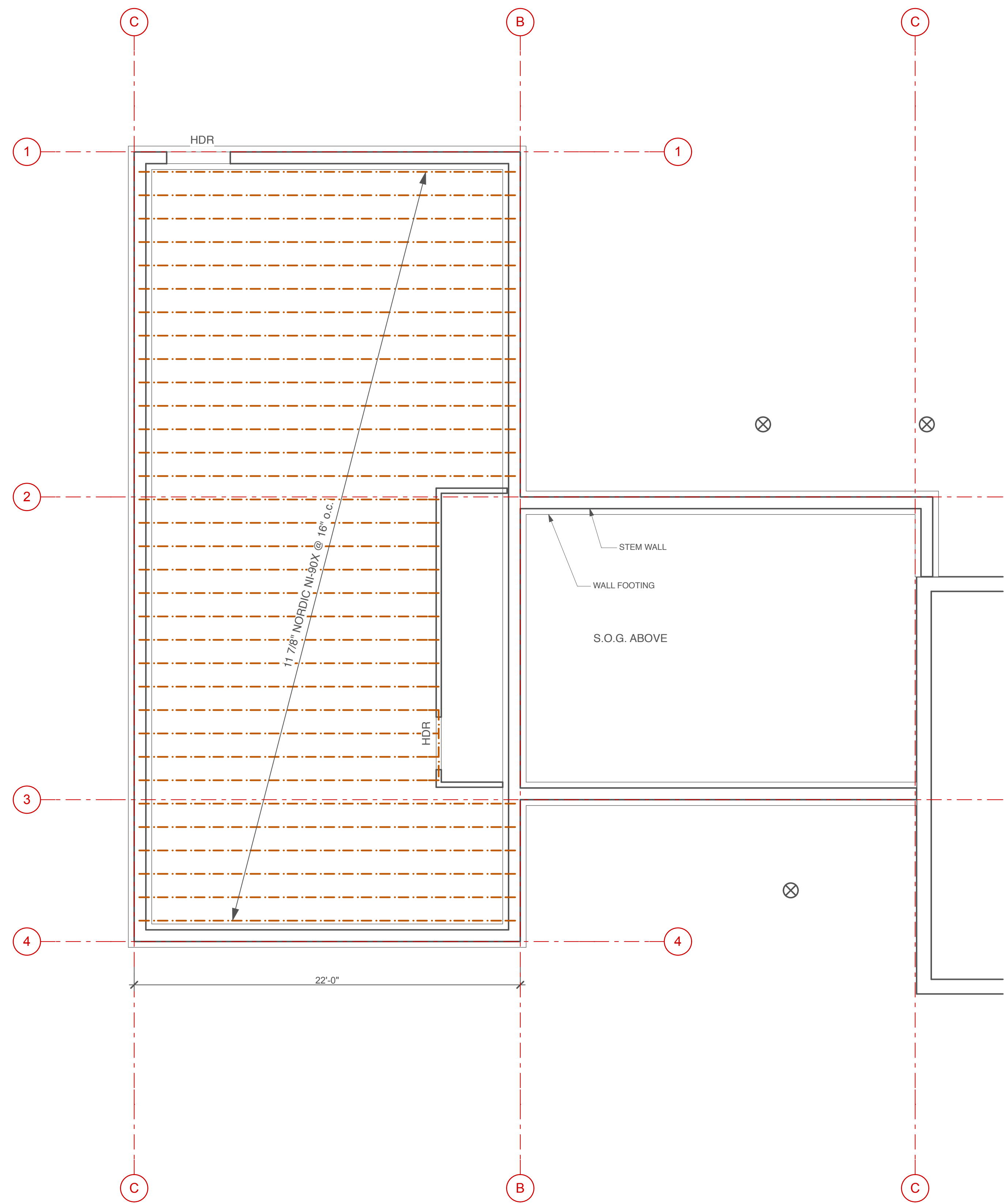
1 1ST FLOOR FRAMING SCALE: 1/4" = 1'-0"
