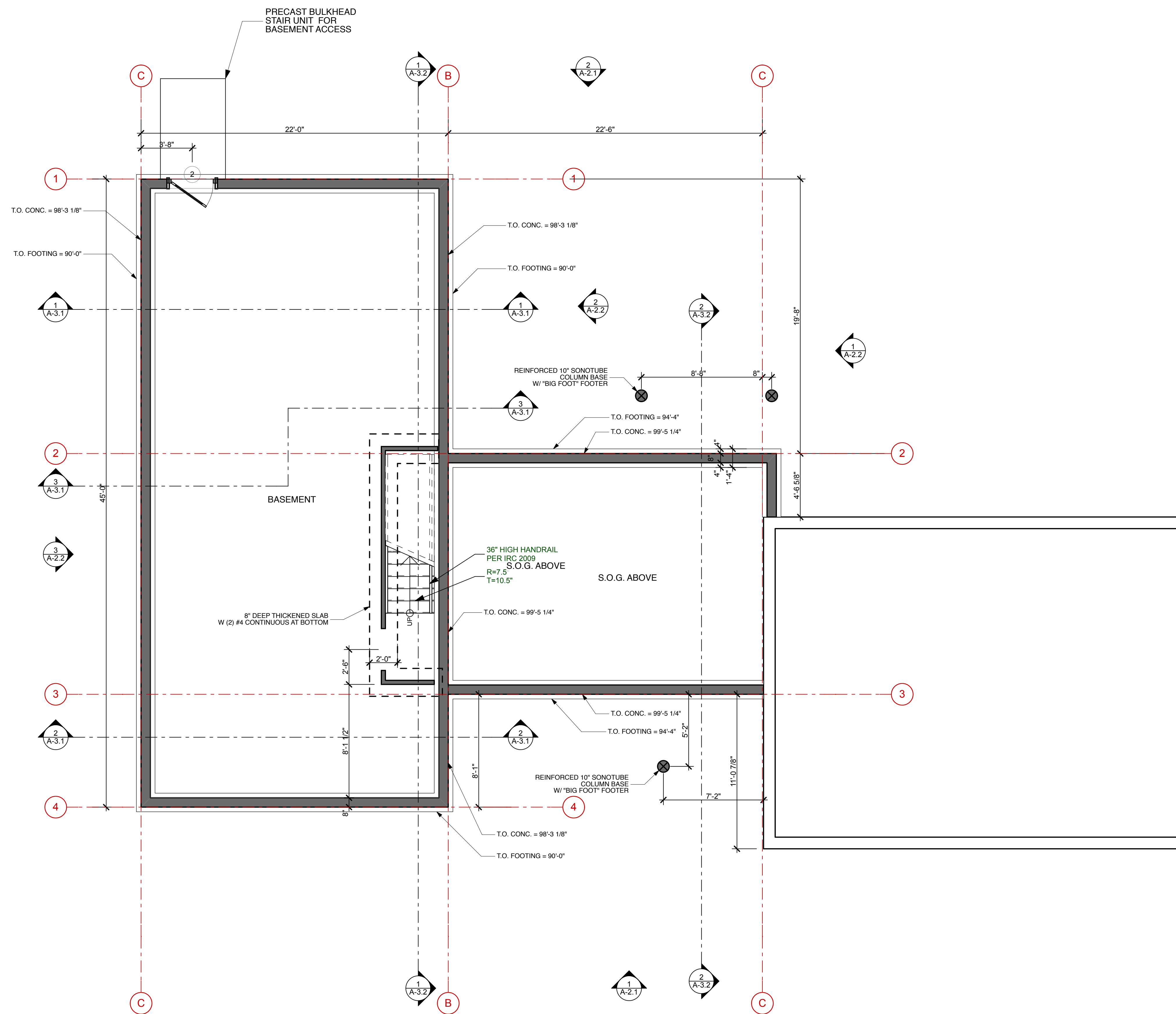
1 FOUNDATION PLAN
