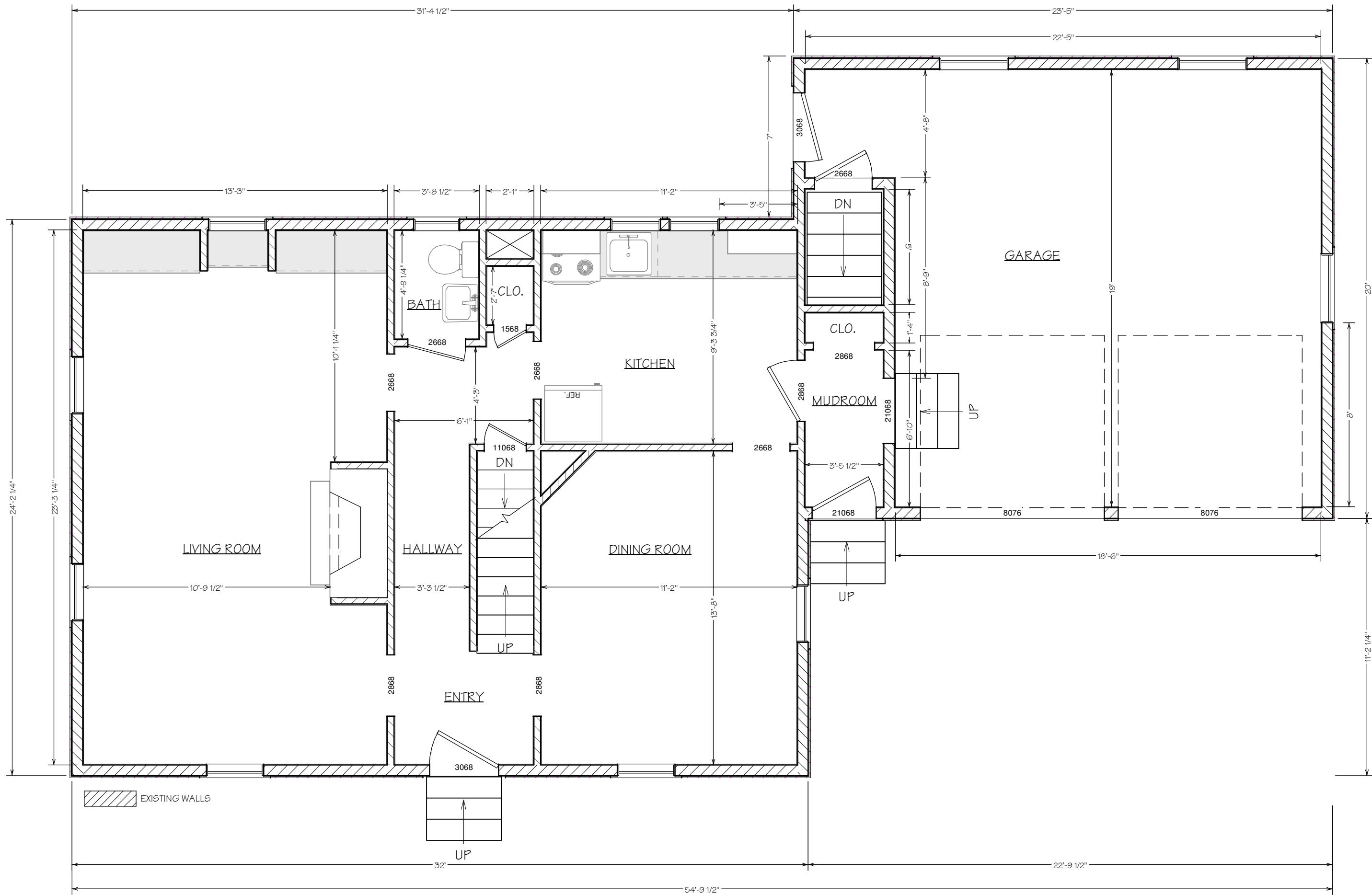
Existing First Floor Plan Scale: 1/4" = 1'-0"
