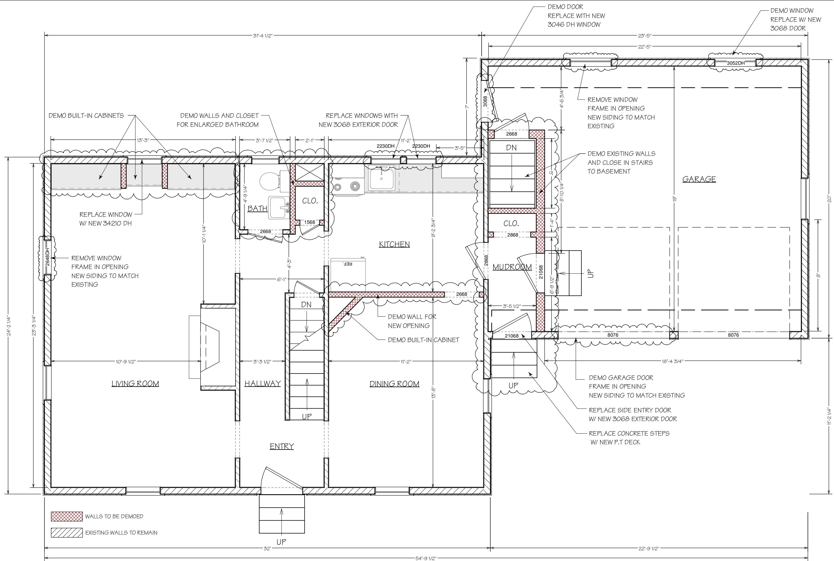
First Floor Demolition Plan Scale: 1/4" = 1'-0"
